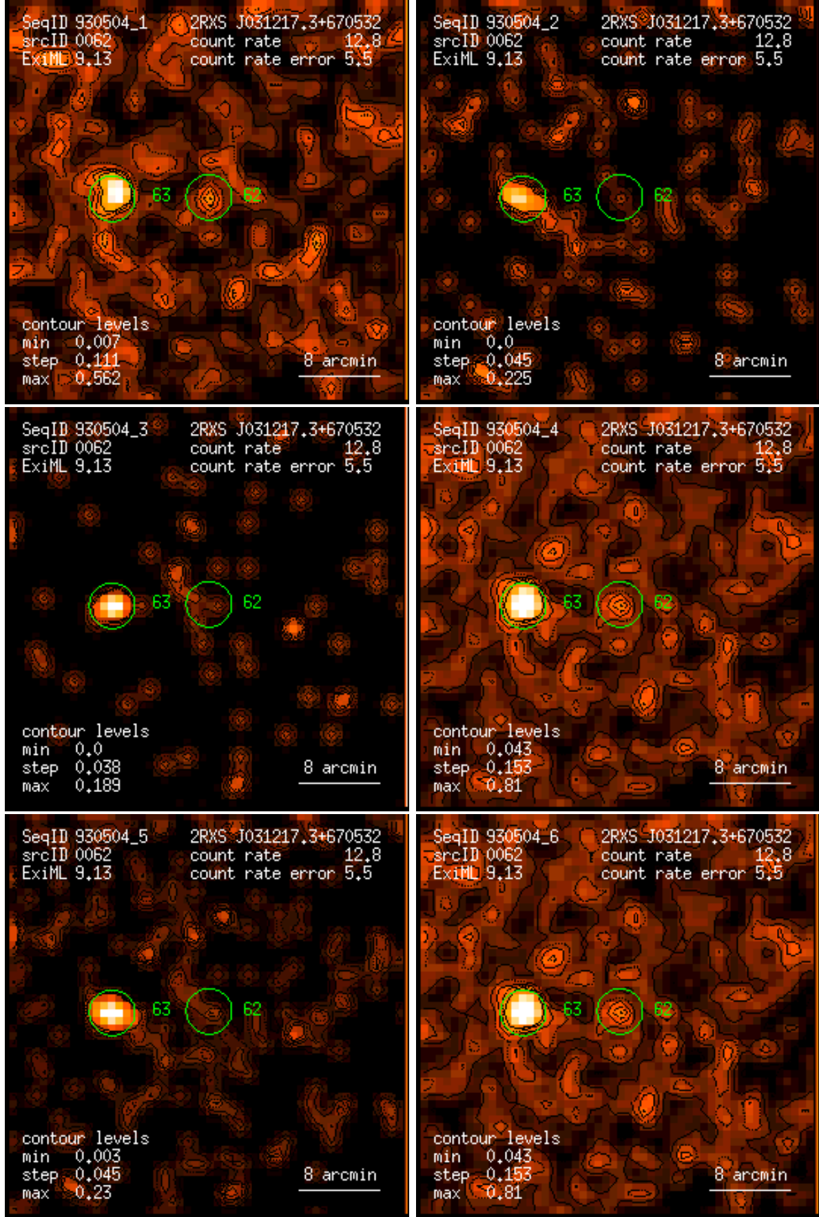
Figure 62: RASS 930504: detection 0062: band rate images, Gaussian filter: (1) PSPC channels 11 – 41, (2) 52 – 90, (3) 91 – 201, (4) 11 – 235, (5) 52 – 201, (6) 11 – 201. Broad band rates in counts/ks. Band rate contour levels in counts/ks/arcmin 2 .
