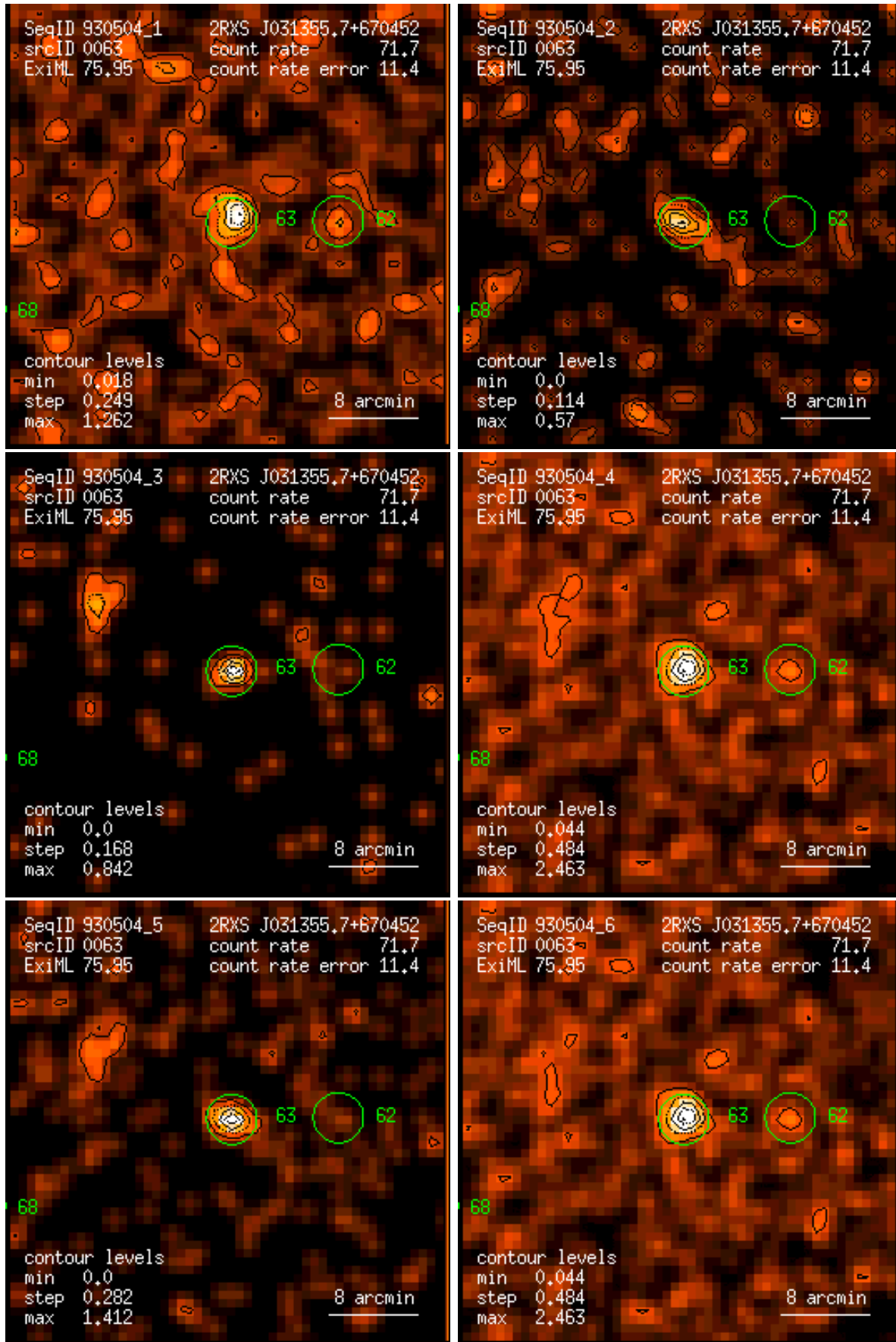
Figure 63: RASS 930504: detection 0063: band rate images, Gaussian filter: (1) PSPC channels 11 – 41, (2) 52 – 90, (3) 91 – 201, (4) 11 – 235, (5) 52 – 201, (6) 11 – 201. Broad band rates in counts/ks. Band rate contour levels in counts/ks/arcmin 2 .
