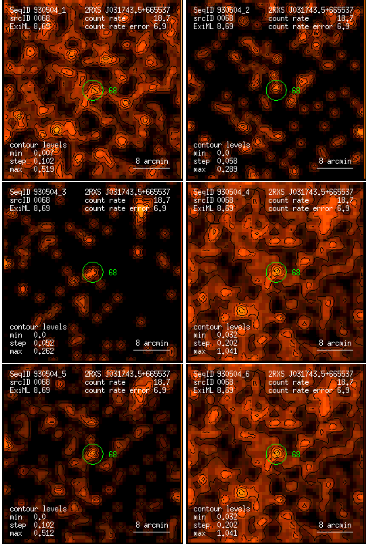
Figure 68: RASS 930504: detection 0068: band rate images, Gaussian filter: (1) PSPC channels 11 – 41, (2) 52 – 90, (3) 91 – 201, (4) 11 – 235, (5) 52 – 201, (6) 11 – 201. Broad band rates in counts/ks. Band rate contour levels in counts/ks/arcmin 2 .
