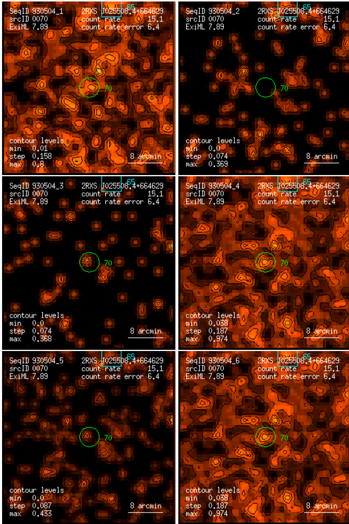
Figure 70: RASS 930504: detection 0070: band rate images, Gaussian filter: (1) PSPC channels 11 – 41, (2) 52 – 90, (3) 91 – 201, (4) 11 – 235, (5) 52 – 201, (6) 11 – 201. Broad band rates in counts/ks. Band rate contour levels in counts/ks/arcmin 2 .
