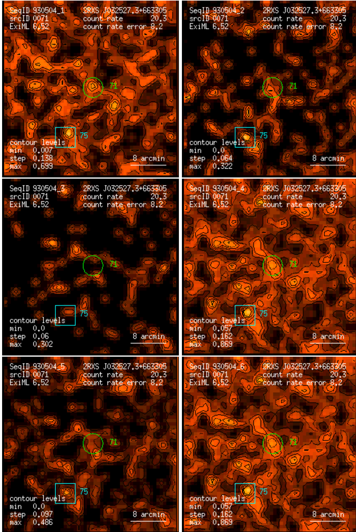
Figure 71: RASS 930504: detection 0071: band rate images, Gaussian filter: (1) PSPC channels 11 – 41, (2) 52 – 90, (3) 91 – 201, (4) 11 – 235, (5) 52 – 201, (6) 11 – 201. Broad band rates in counts/ks. Band rate contour levels in counts/ks/arcmin 2 .
