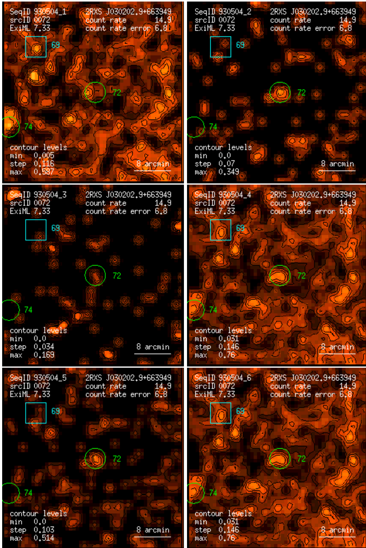
Figure 72: RASS 930504: detection 0072: band rate images, Gaussian filter: (1) PSPC channels 11 – 41, (2) 52 – 90, (3) 91 – 201, (4) 11 – 235, (5) 52 – 201, (6) 11 – 201. Broad band rates in counts/ks. Band rate contour levels in counts/ks/arcmin 2 .
