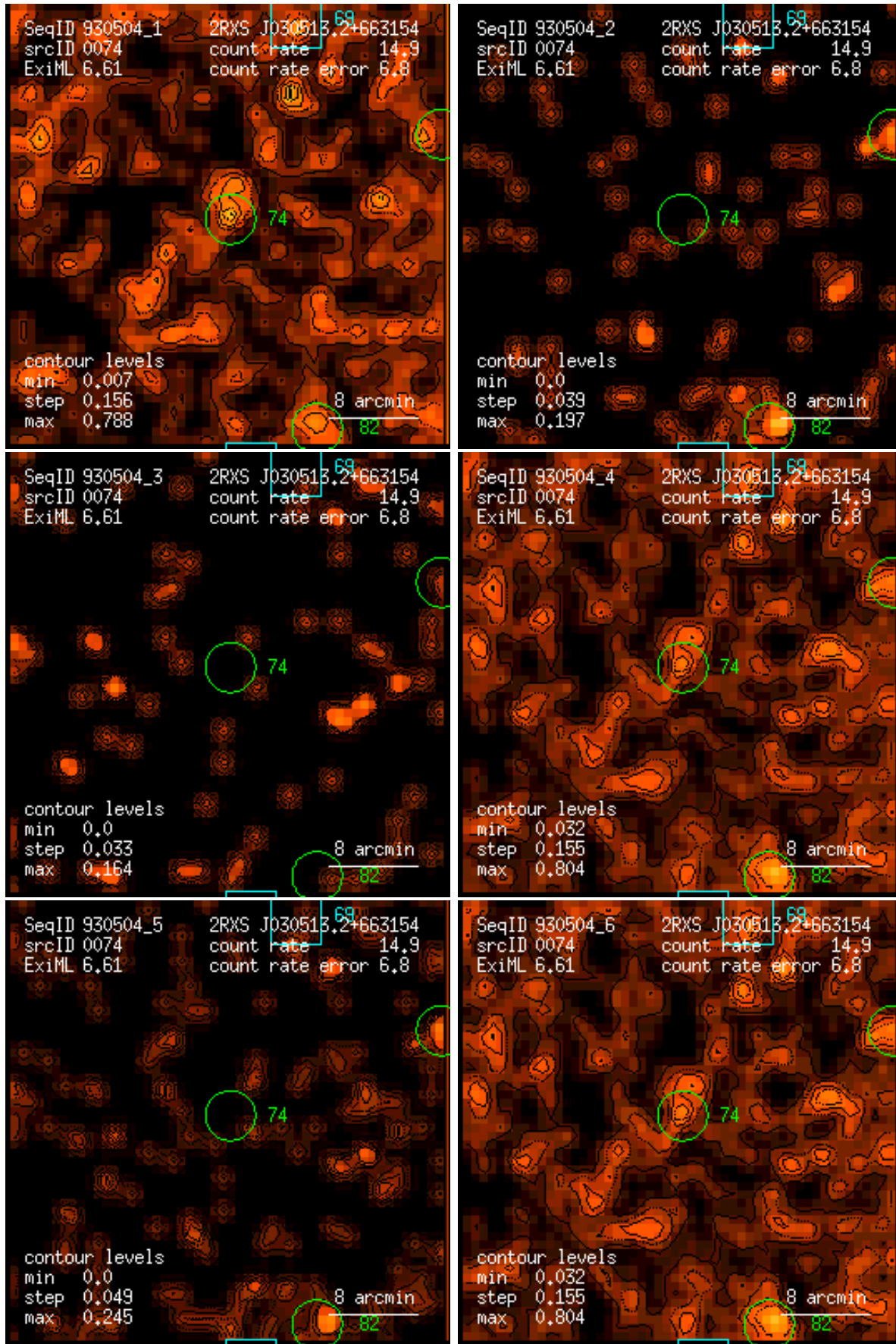
Figure 74: RASS 930504: detection 0074: band rate images, Gaussian filter: (1) PSPC channels 11 – 41, (2) 52 – 90, (3) 91 – 201, (4) 11 – 235, (5) 52 – 201, (6) 11 – 201. Broad band rates in counts/ks. Band rate contour levels in counts/ks/arcmin 2 .
