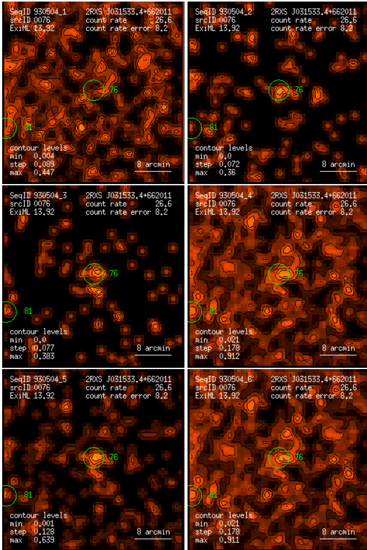
Figure 76: RASS 930504: detection 0076: band rate images, Gaussian filter: (1) PSPP channels 11 – 41, (2) 52 – 90, (3) 91 – 201, (4) 11 – 235, (5) 52 – 201, (6) 11 – 201. Broad band rates in counts/ks. Band rate contour levels in counts/ks/arcmin 2 .
