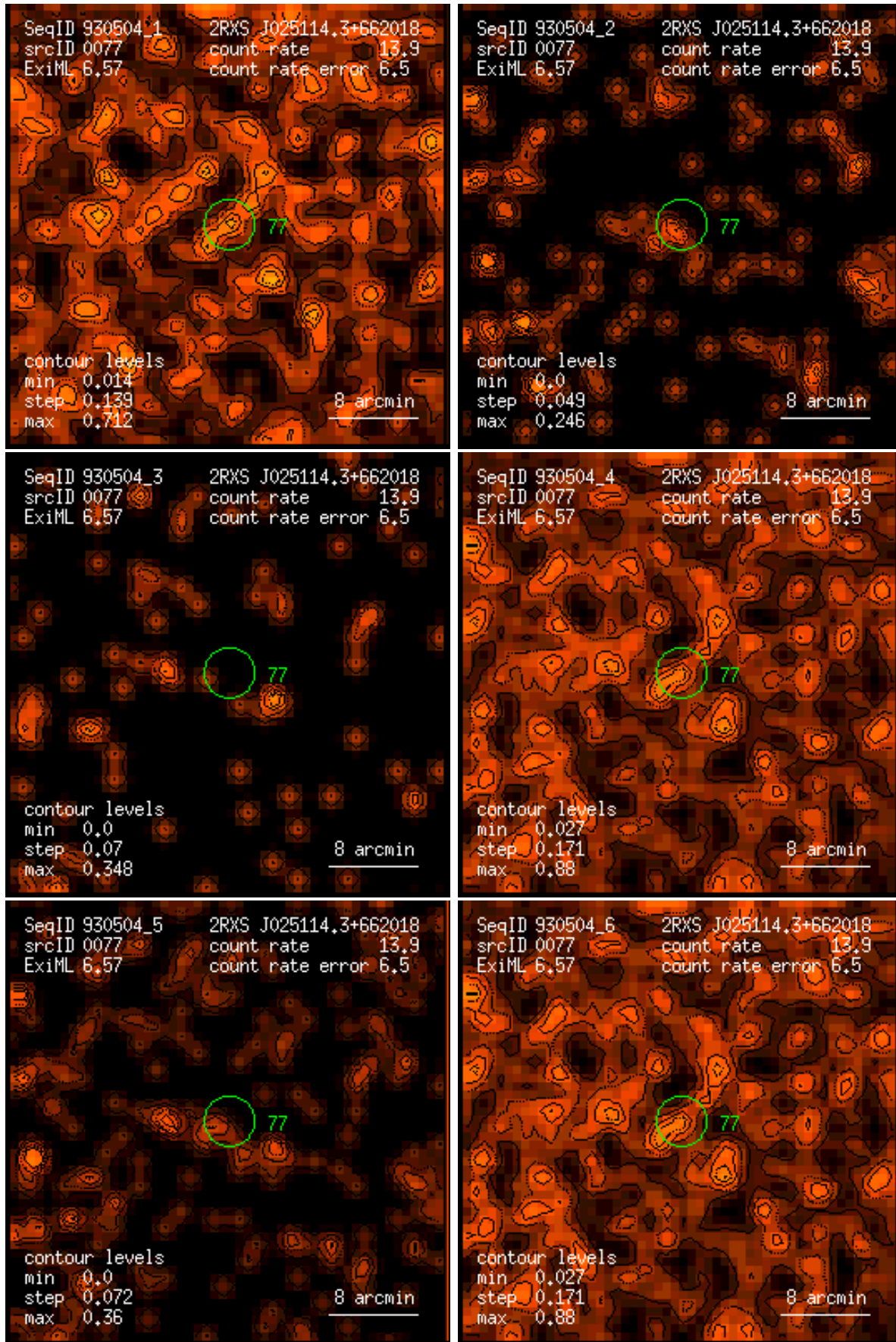
Figure 77: RASS 930504: detection 0077: band rate images, Gaussian filter: (1) PSPC channels 11 – 41, (2) 52 – 90, (3) 91 – 201, (4) 11 – 235, (5) 52 – 201, (6) 11 – 201. Broad band rates in counts/ks. Band rate contour levels in counts/ks/arcmin 2 .
