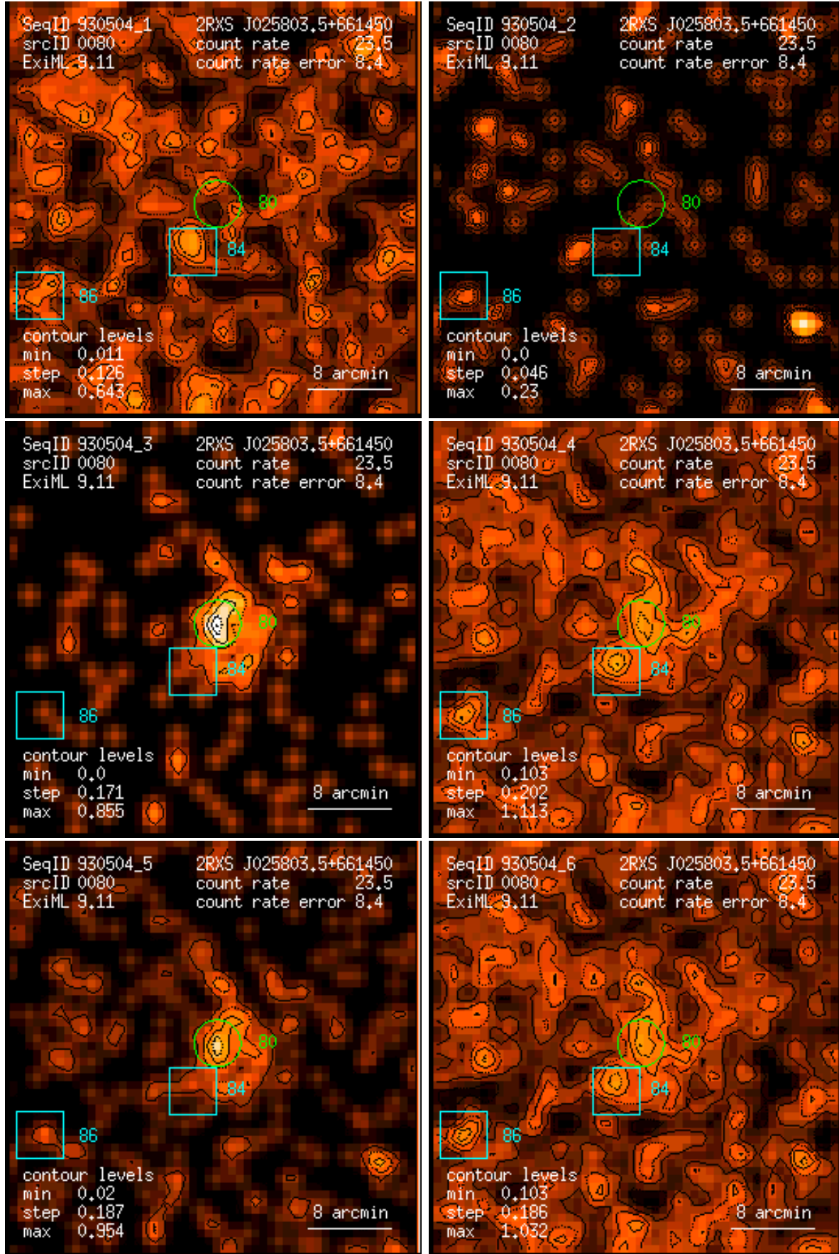
Figure 80: RASS 930504: detection 0080: band rate images, Gaussian filter: (1) PSPC channels 11 – 41, (2) 52 – 90, (3) 91 – 201, (4) 11 – 235, (5) 52 – 201, (6) 11 – 201. Broad band rates in counts/ks. Band rate contour levels in counts/ks/arcmin 2 .
