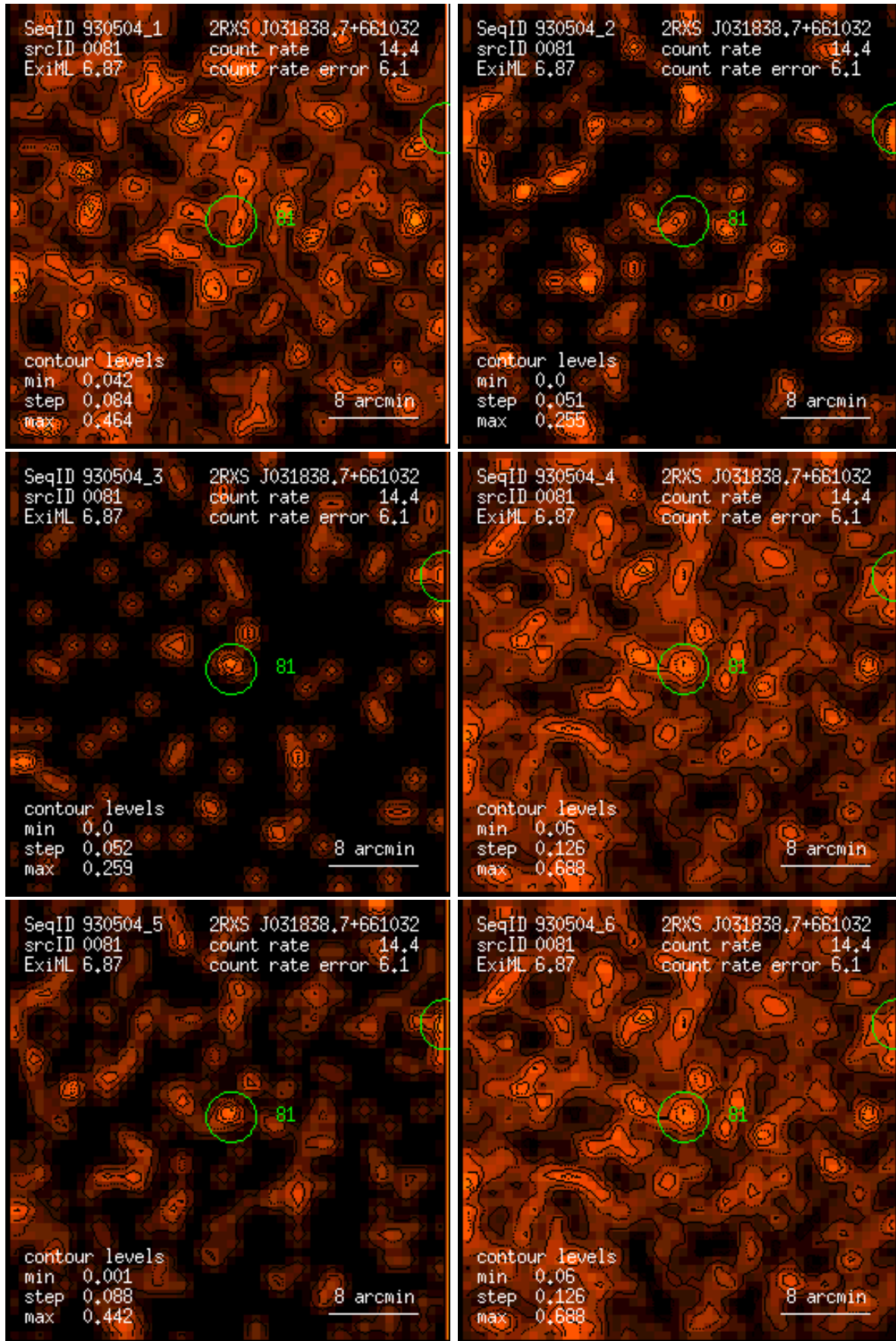
Figure 81: RASS 930504: detection 0081: band rate images, Gaussian filter: (1) PSPC channels 11 – 41, (2) 52 – 90, (3) 91 – 201, (4) 11 – 235, (5) 52 – 201, (6) 11 – 201. Broad band rates in counts/ks. Band rate contour levels in counts/ks/arcmin 2 .
