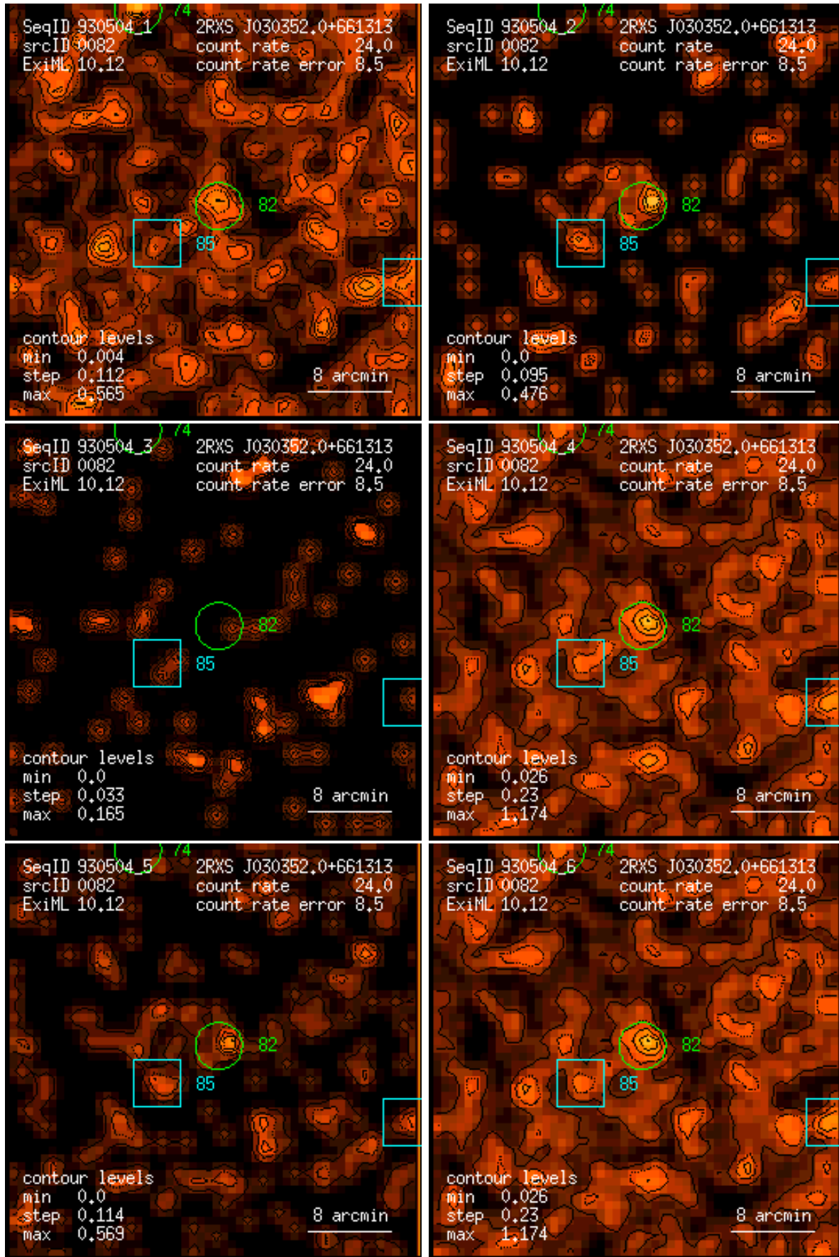
Figure 82: RASS 930504: detection 0082: band rate images, Gaussian filter: (1) PSPC channels 11 – 41, (2) 52 – 90, (3) 91 – 201, (4) 11 – 235, (5) 52 – 201, (6) 11 – 201. Broad band rates in counts/ks. Band rate contour levels in counts/ks/arcmin 2 .
