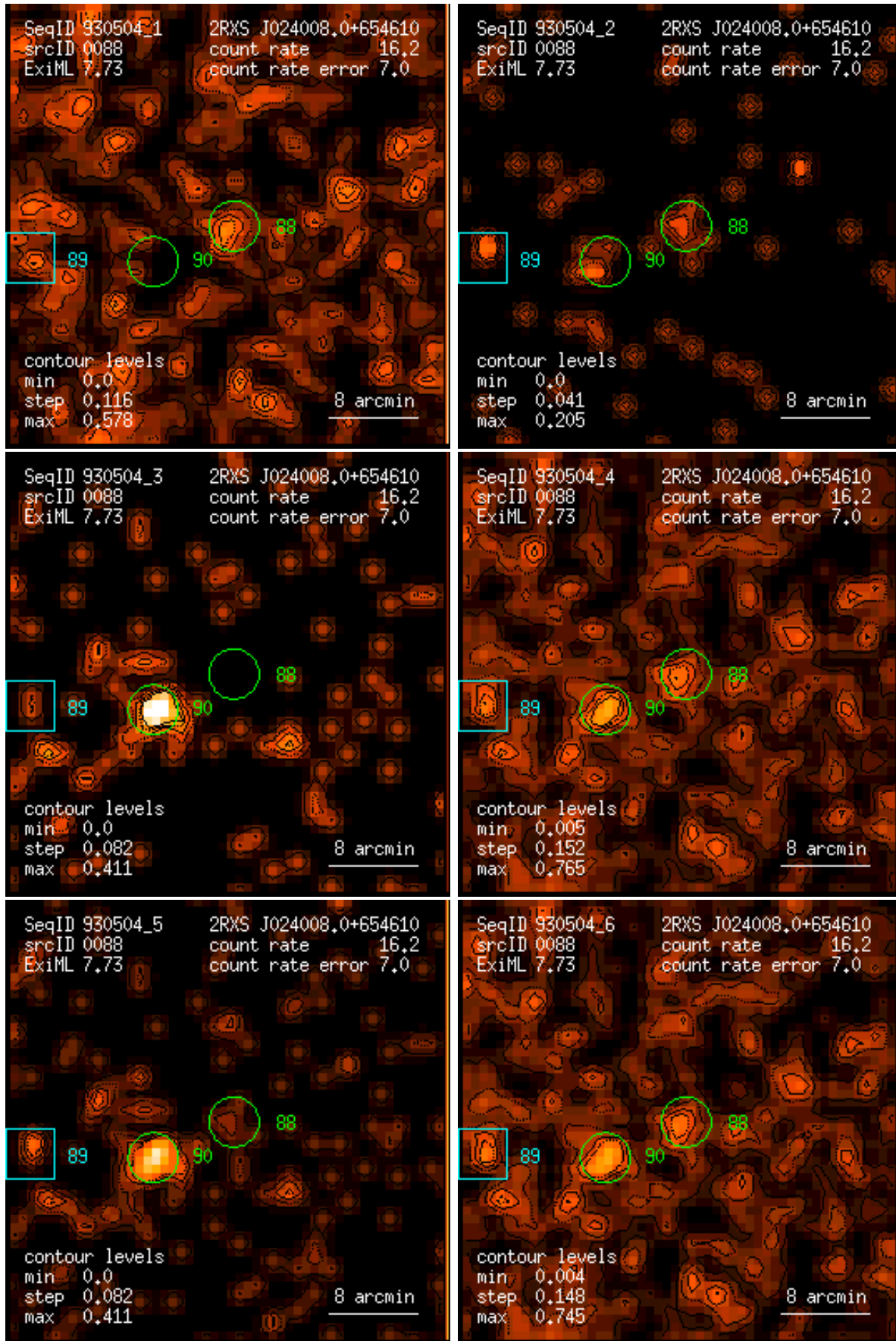
Figure 88: RASS 930504: detection 0088: band rate images, Gaussian filter: (1) PSPC channels 11 – 41, (2) 52 – 90, (3) 91 – 201, (4) 11 – 235, (5) 52 – 201, (6) 11 – 201. Broad band rates in counts/ks. Band rate contour levels in counts/ks/arcmin 2 .
