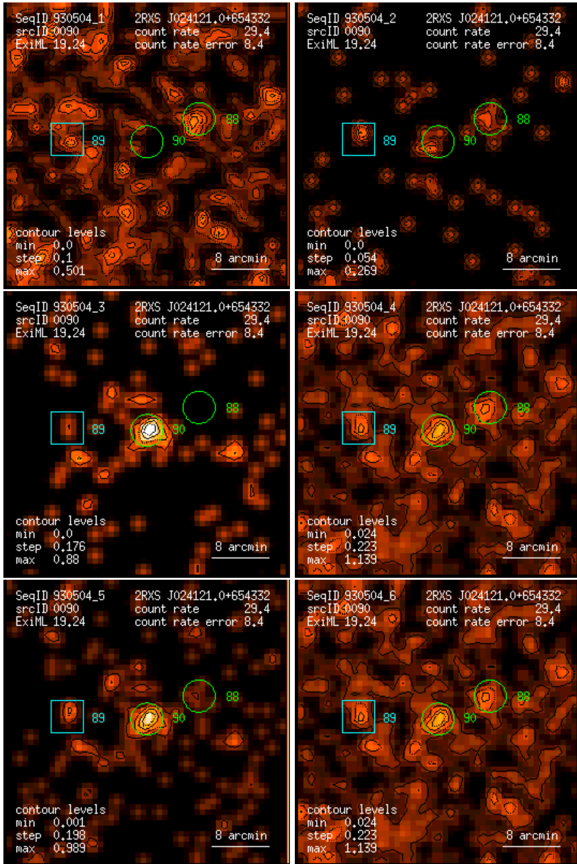
Figure 90: RASS 930504: detection 0090: band rate images, Gaussian filter: (1) PSPC channels 11 – 41, (2) 52 – 90, (3) 91 – 201, (4) 11 – 235, (5) 52 – 201, (6) 11 – 201. Broad band rates in counts/ks. Band rate contour levels in counts/ks/arcmin 2 .
