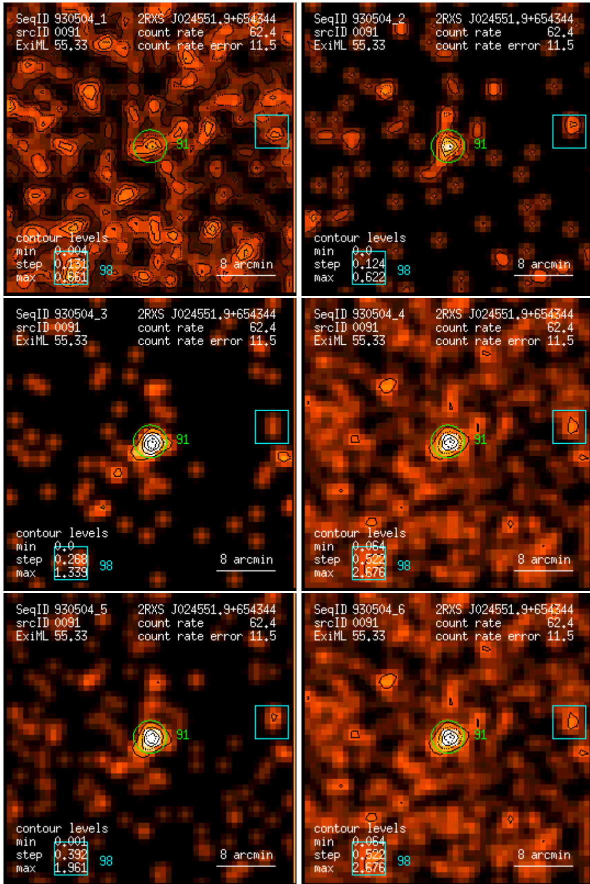
Figure 91: RASS 930504: detection 0091: band rate images, Gaussian filter: (1) PSPC channels 11 – 41, (2) 52 – 90, (3) 91 – 201, (4) 11 – 235, (5) 52 – 201, (6) 11 – 201. Broad band rates in counts/ks. Band rate contour levels in counts/ks/arcmin 2 .
