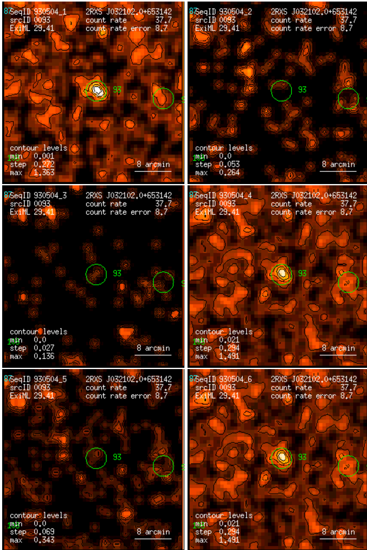
Figure 93: RASS 930504: detection 0093: band rate images, Gaussian filter: (1) PSPC channels 11 – 41, (2) 52 – 90, (3) 91 – 201, (4) 11 – 235, (5) 52 – 201, (6) 11 – 201. Broad band rates in counts/ks. Band rate contour levels in counts/ks/arcmin 2 .
