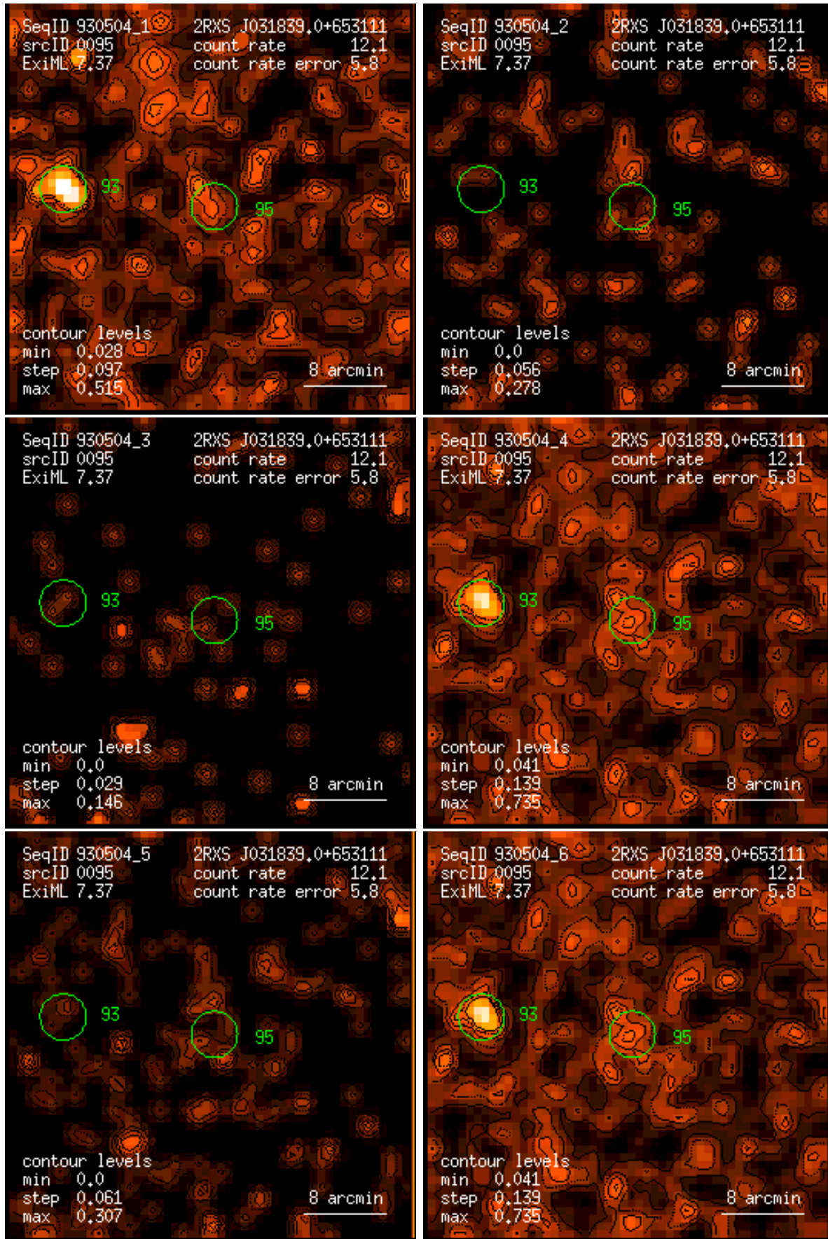
Figure 95: RASS 930504: detection 0095: band rate images, Gaussian filter: (1) PSPC channels 11 – 41, (2) 52 – 90, (3) 91 – 201, (4) 11 – 235, (5) 52 – 201, (6) 11 – 201. Broad band rates in counts/ks. Band rate contour levels in counts/ks/arcmin 2 .
