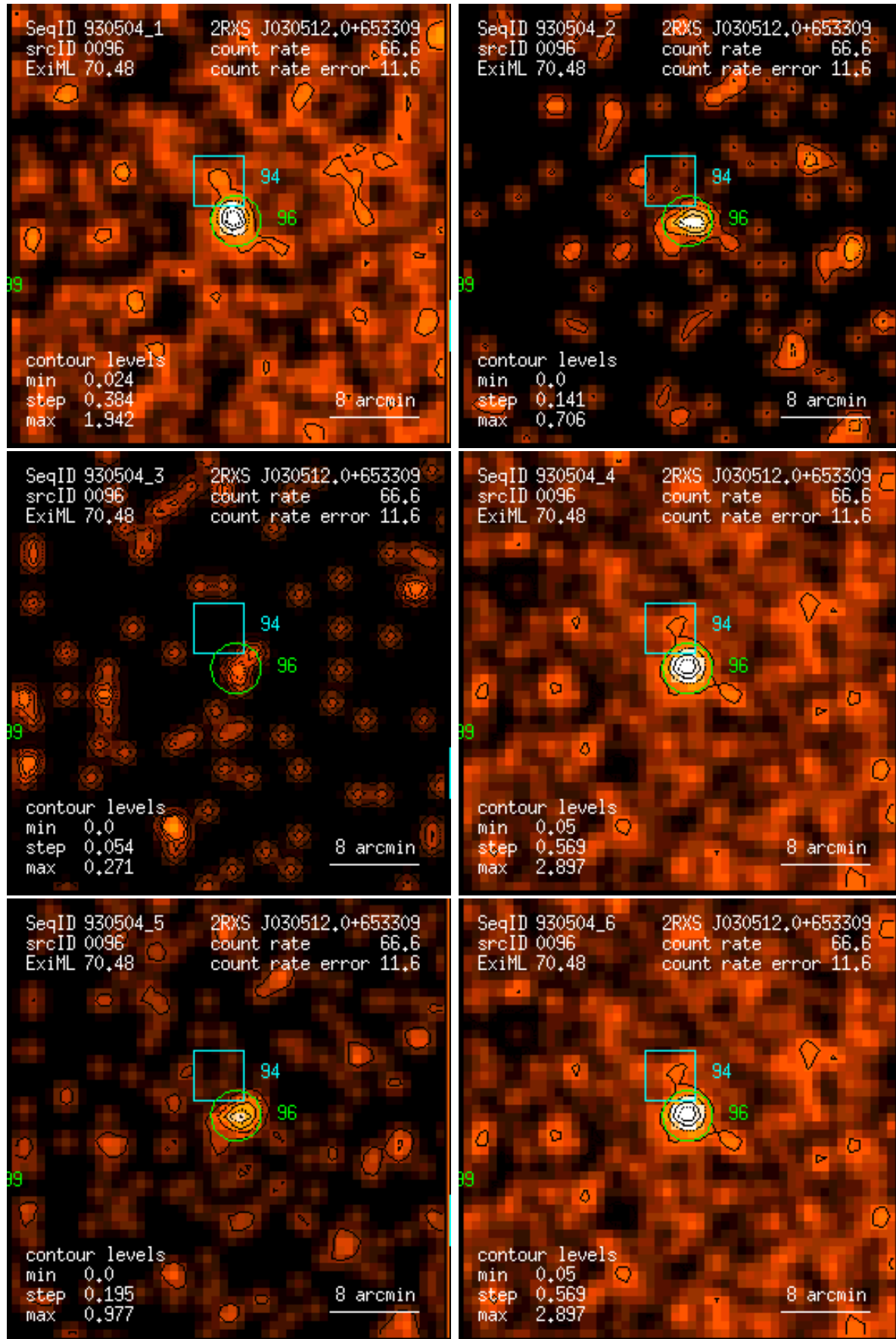
Figure 96: RASS 930504: detection 0096: band rate images, Gaussian filter: (1) PSPC channels 11 – 41, (2) 52 – 90, (3) 91 – 201, (4) 11 – 235, (5) 52 – 201, (6) 11 – 201. Broad band rates in counts/ks. Band rate contour levels in counts/ks/arcmin 2 .
