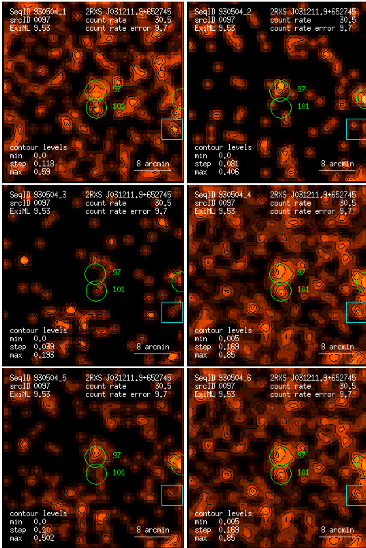
Figure 97: RASS 930504: detection 0097: band rate images, Gaussian filter: (1) PSPC channels 11 – 41, (2) 52 – 90, (3) 91 – 201, (4) 11 – 235, (5) 52 – 201, (6) 11 – 201. Broad band rates in counts/ks. Band rate contour levels in counts/ks/arcmin 2 .
