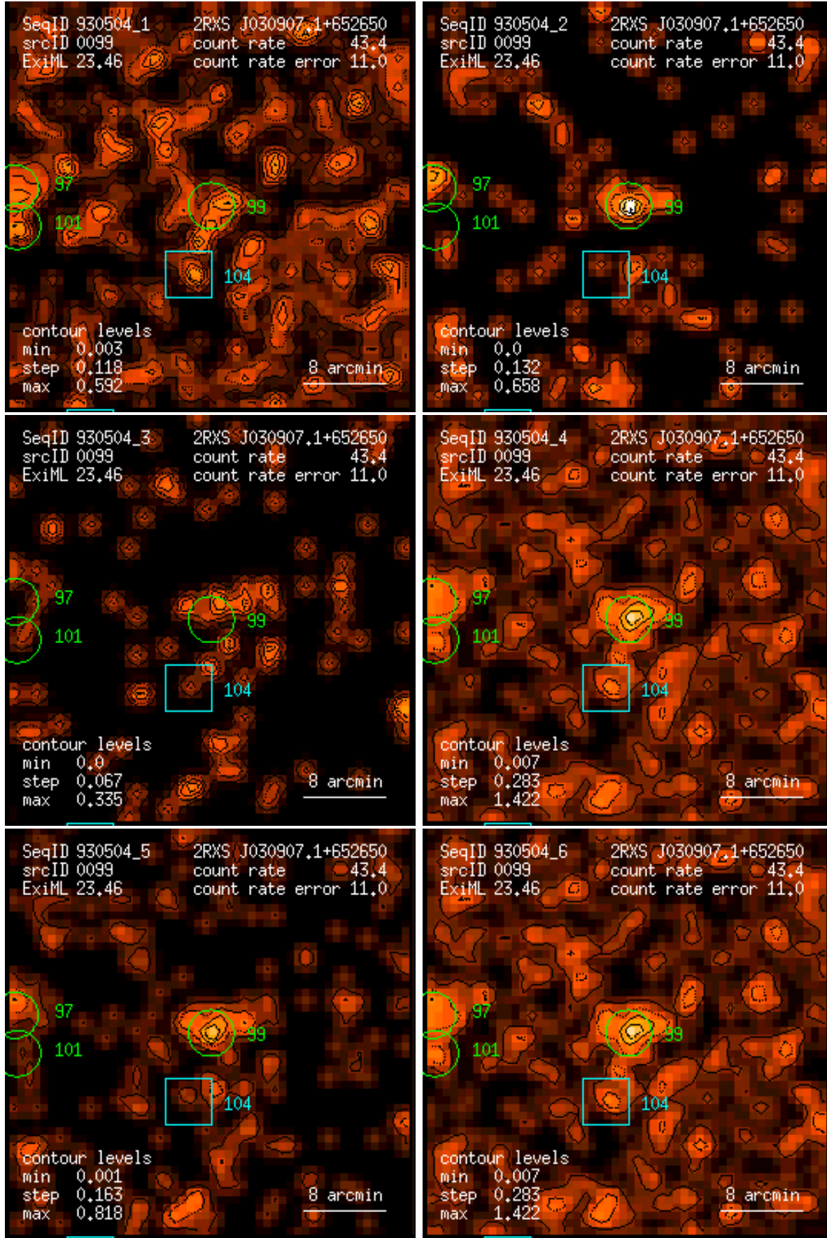
Figure 99: RASS 930504: detection 0099: band rate images, Gaussian filter: (1) PSPC channels 11 – 41, (2) 52 – 90, (3) 91 – 201, (4) 11 – 235, (5) 52 – 201, (6) 11 – 201. Broad band rates in counts/ks. Band rate contour levels in counts/ks/arcmin 2 .
