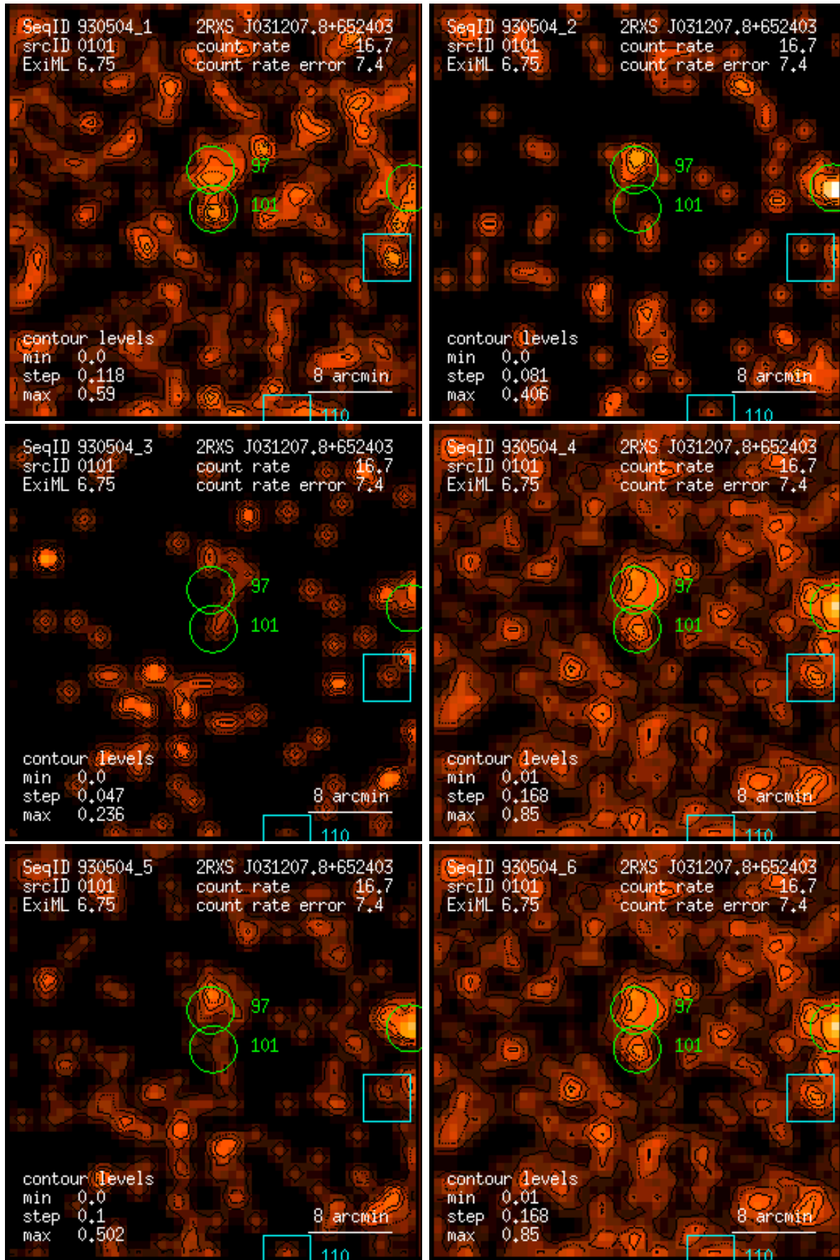
Figure 101: RASS 930504: detection 0101: band rate images, Gaussian filter: (1) PSPC channels 11 – 41, (2) 52 – 90, (3) 91 – 201, (4) 11 – 235, (5) 52 – 201, (6) 11 – 201. Broad band rates in counts/ks. Band rate contour levels in counts/ks/arcmin 2 .
