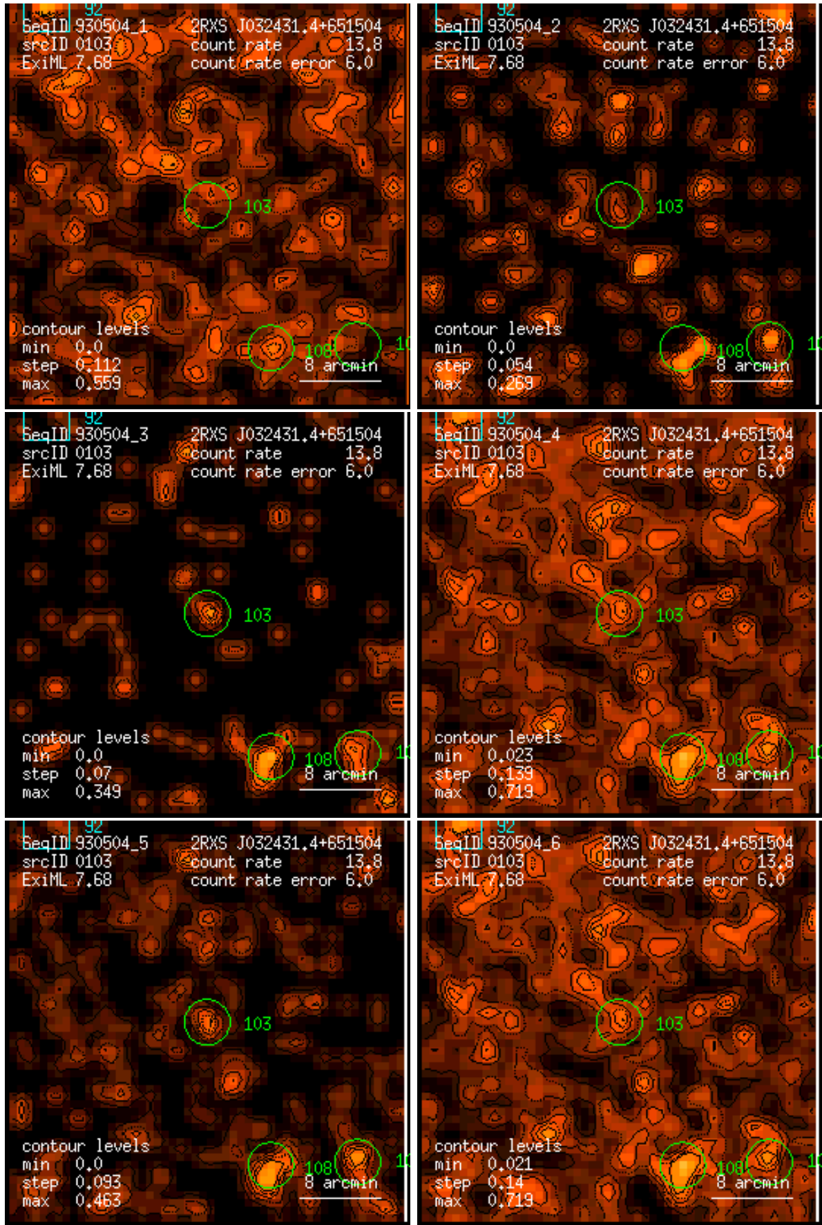
Figure 103: RASS 930504: detection 0103: band rate images, Gaussian filter: (1) PSPC channels 11 – 41, (2) 52 – 90, (3) 91 – 201, (4) 11 – 235, (5) 52 – 201, (6) 11 – 201. Broad band rates in counts/ks. Band rate contour levels in counts/ks/arcmin 2 .
