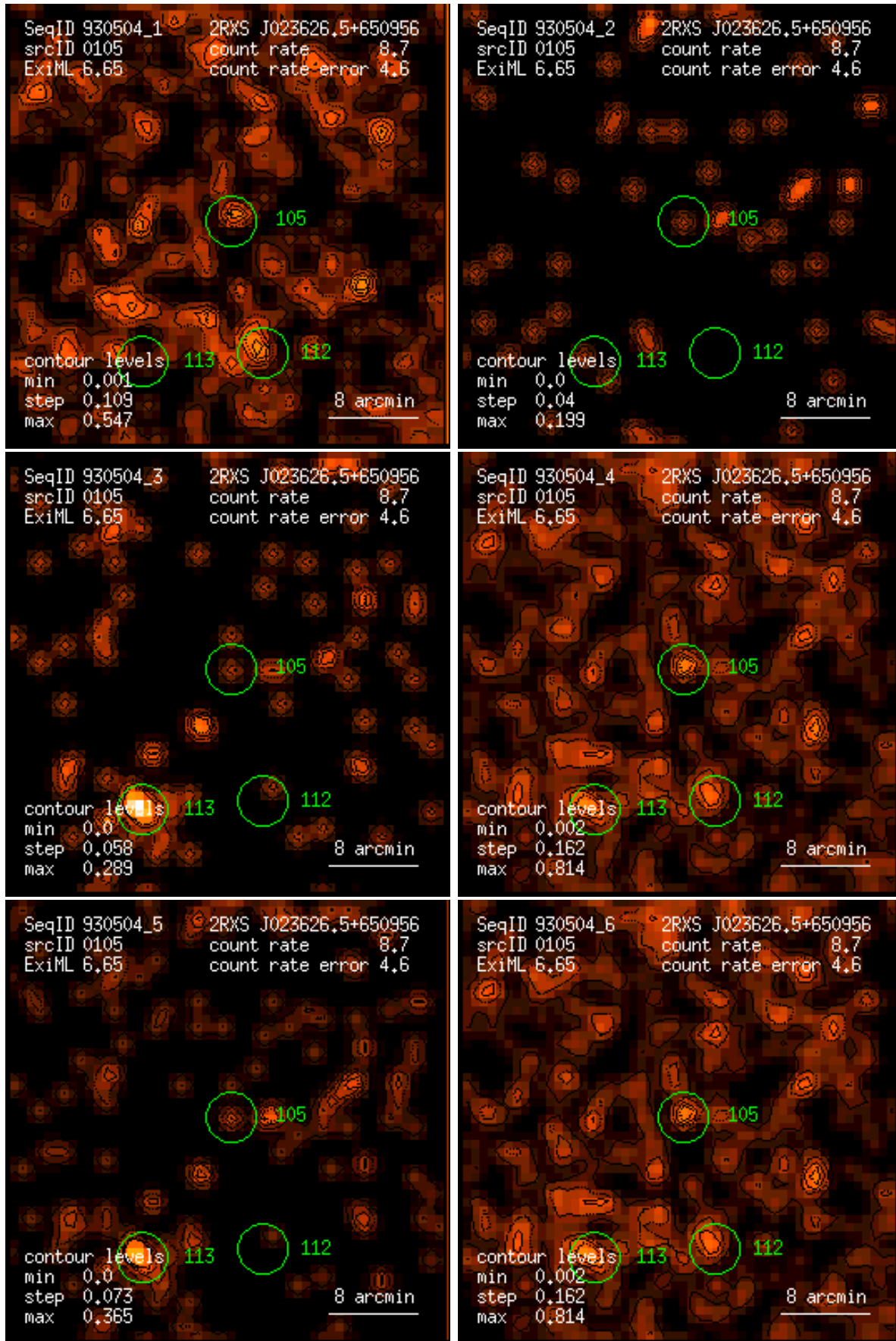
Figure 105: RASS 930504: detection 0105: band rate images, Gaussian filter: (1) PSPC channels 11 – 41, (2) 52 – 90, (3) 91 – 201, (4) 11 – 235, (5) 52 – 201, (6) 11 – 201. Broad band rates in counts/ks. Band rate contour levels in counts/ks/arcmin 2 .
