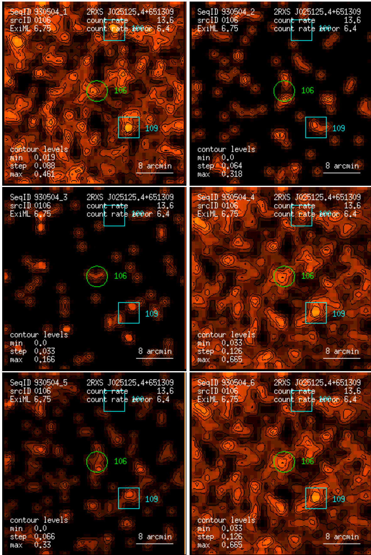
Figure 106: RASS 930504: detection 0106: band rate images, Gaussian filter: (1) PSPC channels 11 – 41, (2) 52 – 90, (3) 91 – 201, (4) 11 – 235, (5) 52 – 201, (6) 11 – 201. Broad band rates in counts/ks. Band rate contour levels in counts/ks/arcmin 2 .
