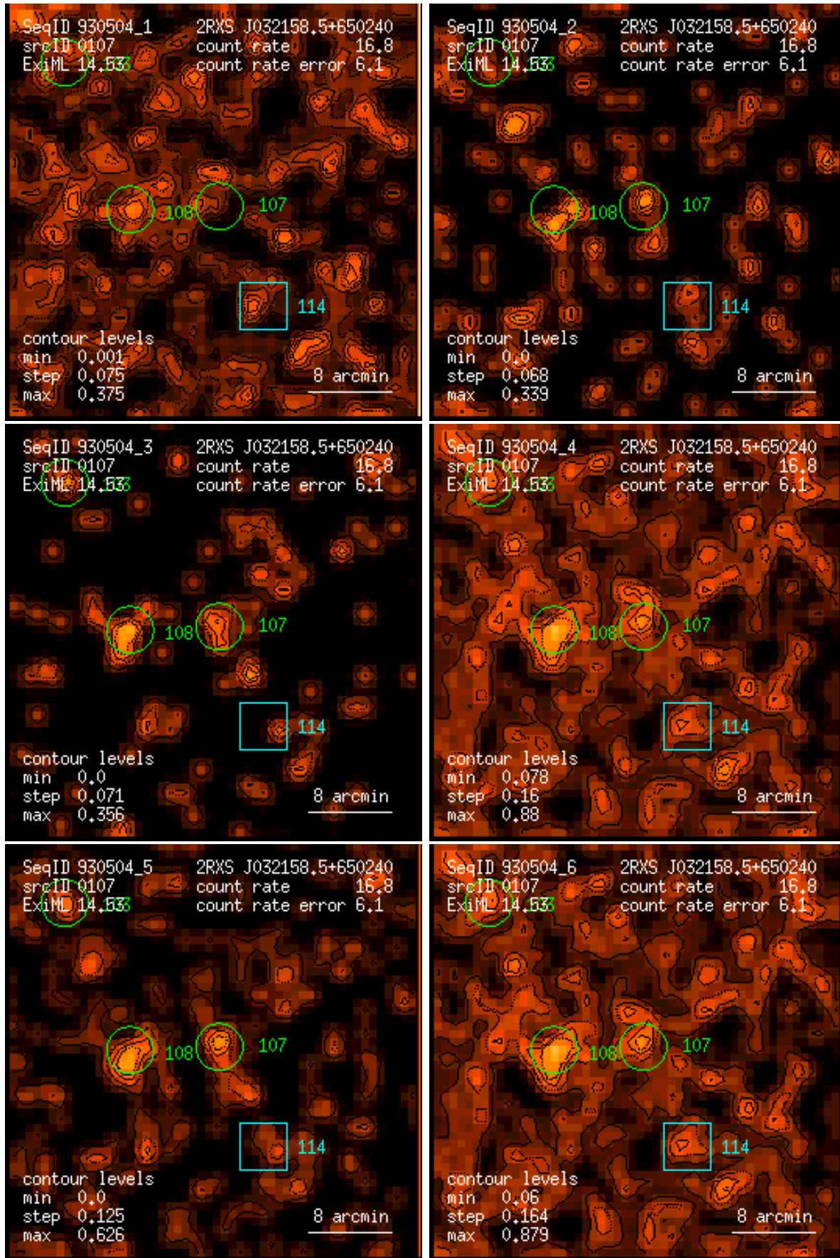
Figure 107: RASS 930504: detection 0107: band rate images, Gaussian filter: (1) PSPC channels 11 – 41, (2) 52 – 90, (3) 91 – 201, (4) 11 – 235, (5) 52 – 201, (6) 11 – 201. Broad band rates in counts/ks. Band rate contour levels in counts/ks/arcmin 2 .
