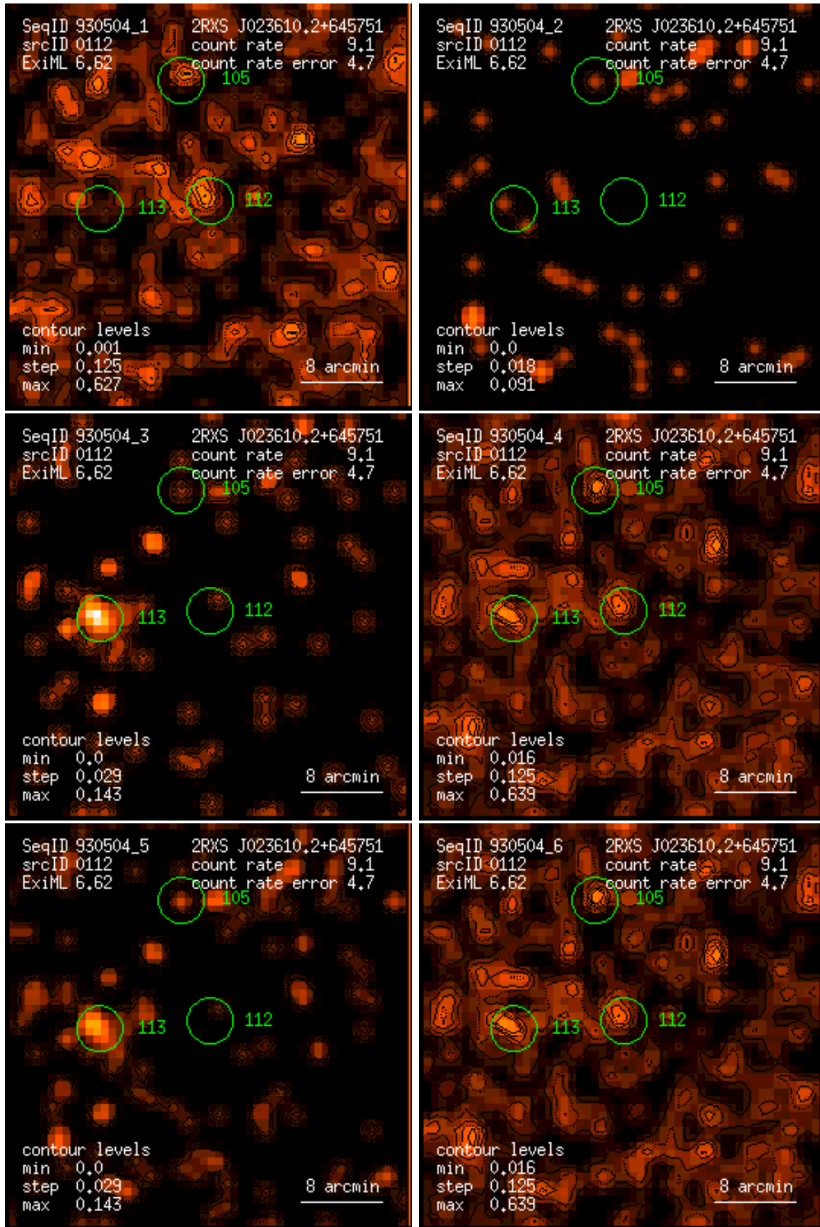
Figure 112: RASS 930504: detection 0112: band rate images, Gaussian filter: (1) PSPC channels 11 – 41, (2) 52 – 90, (3) 91 – 201, (4) 11 – 235, (5) 52 – 201, (6) 11 – 201. Broad band rates in counts/ks. Band rate contour levels in counts/ks/arcmin 2 .
