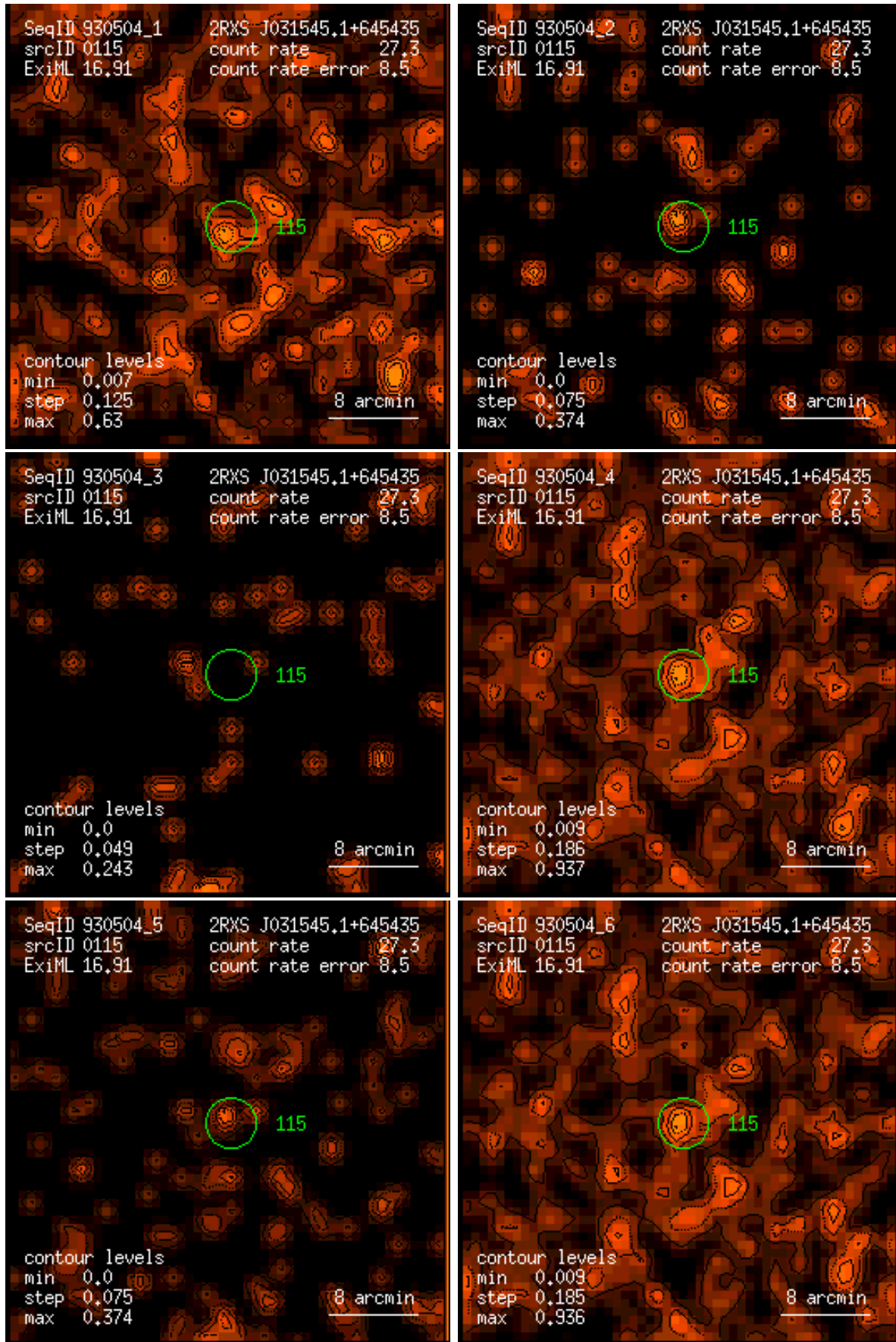
Figure 115: RASS 930504: detection 0115: band rate images, Gaussian filter: (1) PSPC channels 11 – 41, (2) 52 – 90, (3) 91 – 201, (4) 11 – 235, (5) 52 – 201, (6) 11 – 201. Broad band rates in counts/ks. Band rate contour levels in counts/ks/arcmin 2 .
