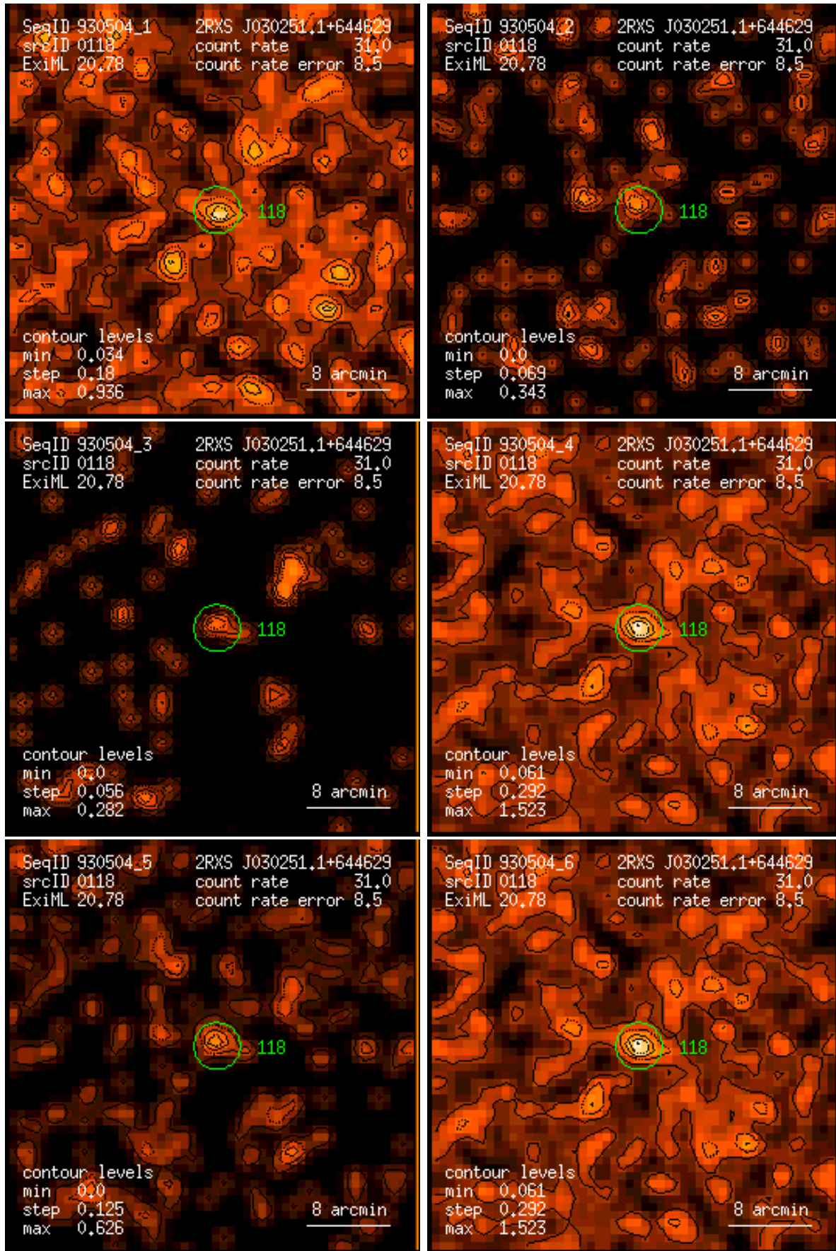
Figure 118: RASS 930504: detection 0118: band rate images, Gaussian filter: (1) PSPC channels 11 – 41, (2) 52 – 90, (3) 91 – 201, (4) 11 – 235, (5) 52 – 201, (6) 11 – 201. Broad band rates in counts/ks. Band rate contour levels in counts/ks/arcmin 2 .
