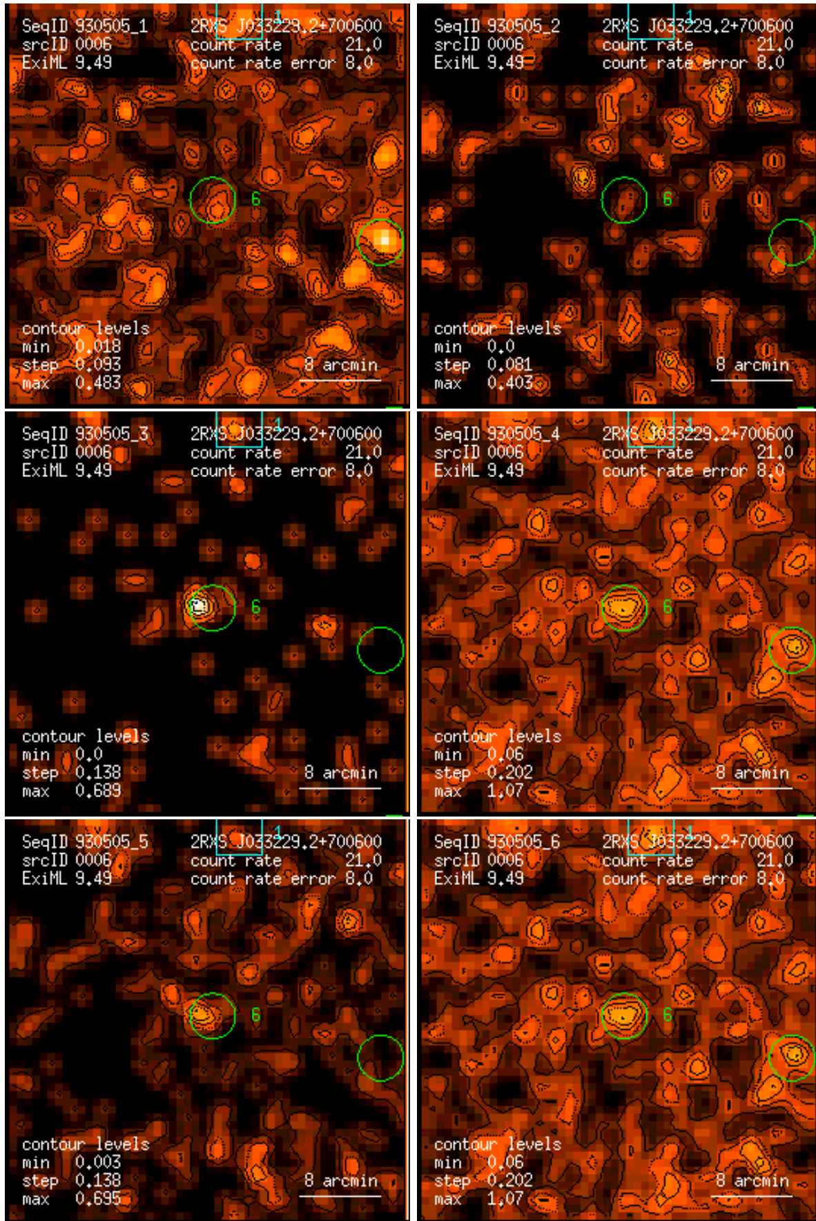
Figure 6: RASS 930505: detection 0006: band rate images, Gaussian filter: (1) PSPC channels 11 – 41, (2) 52 – 90, (3) 91 – 201, (4) 11 – 235, (5) 52 – 201, (6) 11 – 201. Broad band rates in counts/ks. Band rate contour levels in counts/ks/arcmin 2 .
