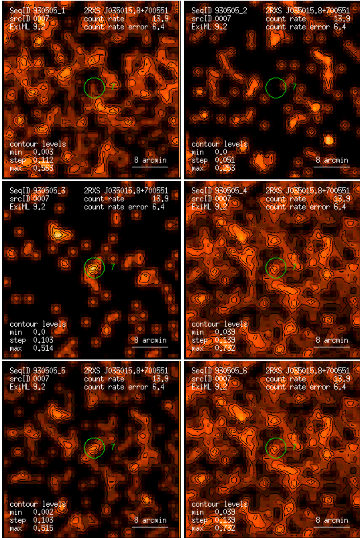
Figure 7: RASS 930505: detection 0007: band rate images, Gaussian filter: (1) PSPC channels 11 – 41, (2) 52 – 90, (3) 91 – 201, (4) 11 – 235, (5) 52 – 201, (6) 11 – 201. Broad band rates in counts/ks. Band rate contour levels in counts/ks/arcmin 2 .
