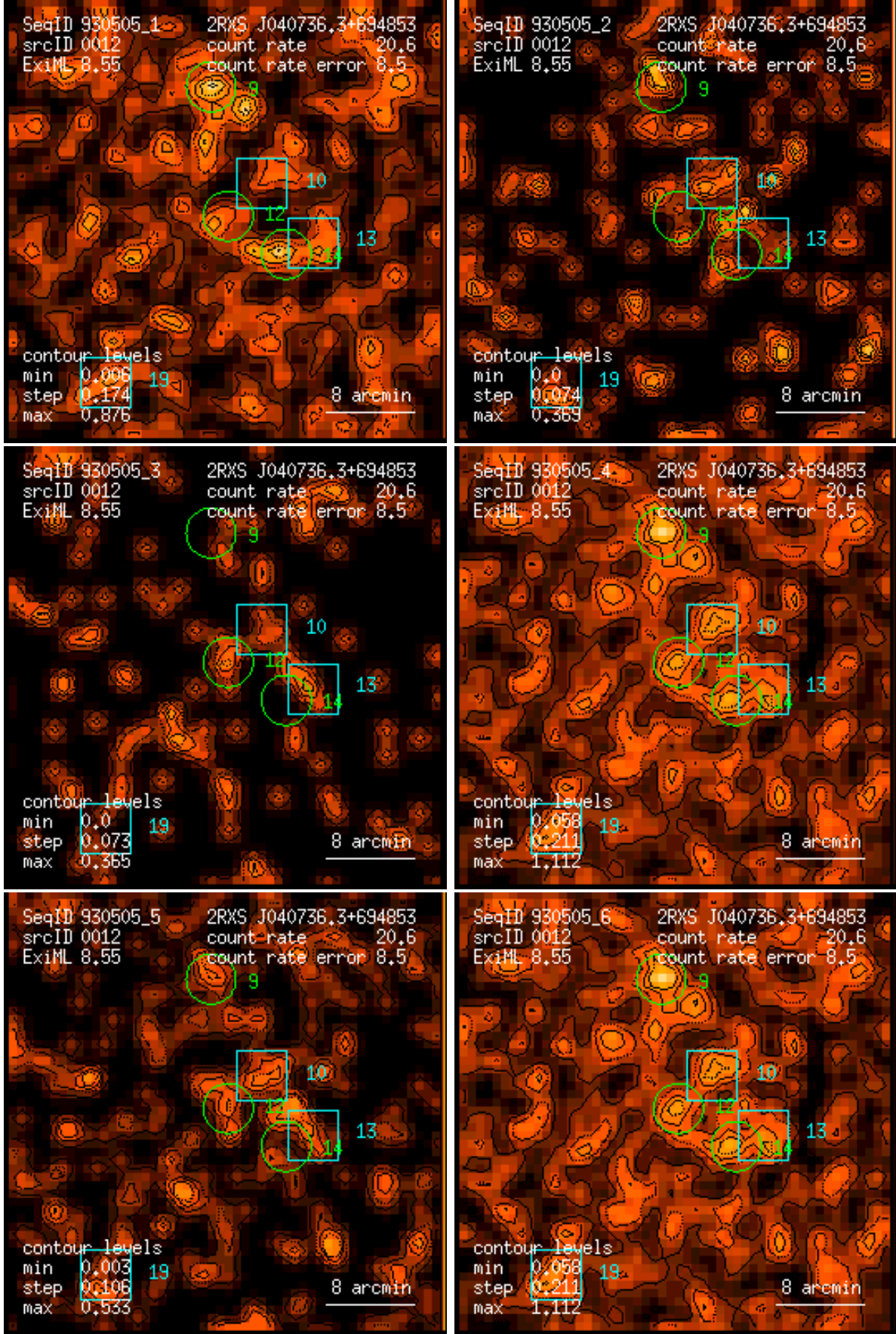
Figure 12: RASS 930505: detection 0012: band rate images, Gaussian filter: (1) PSPC channels 11 – 41, (2) 52 – 90, (3) 91 – 201, (4) 11 – 235, (5) 52 – 201, (6) 11 – 201. Broad band rates in counts/ks. Band rate contour levels in counts/ks/arcmin 2 .
