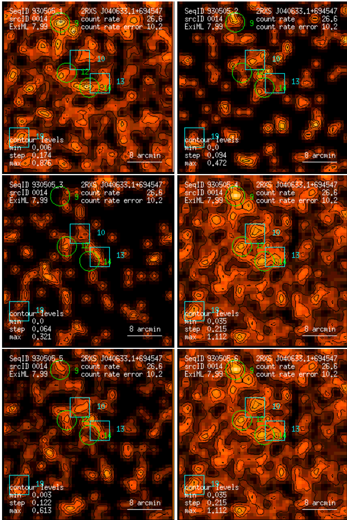
Figure 14: RASS 930505: detection 0014: band rate images, Gaussian filter: (1) PSPC channels 11 – 41, (2) 52 – 90, (3) 91 – 201, (4) 11 – 235, (5) 52 – 201, (6) 11 – 201. Broad band rates in counts/ks. Band rate contour levels in counts/ks/arcmin 2 .
