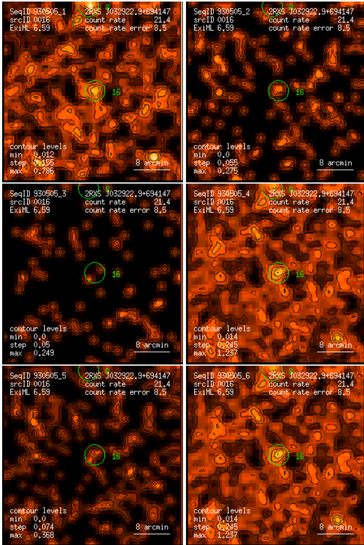
Figure 16: RASS 930505: detection 0016: band rate images, Gaussian filter: (1) PSPC channels 11 – 41, (2) 52 – 90, (3) 91 – 201, (4) 11 – 235, (5) 52 – 201, (6) 11 – 201. Broad band rates in counts/ks. Band rate contour levels in counts/ks/arcmin 2 .
