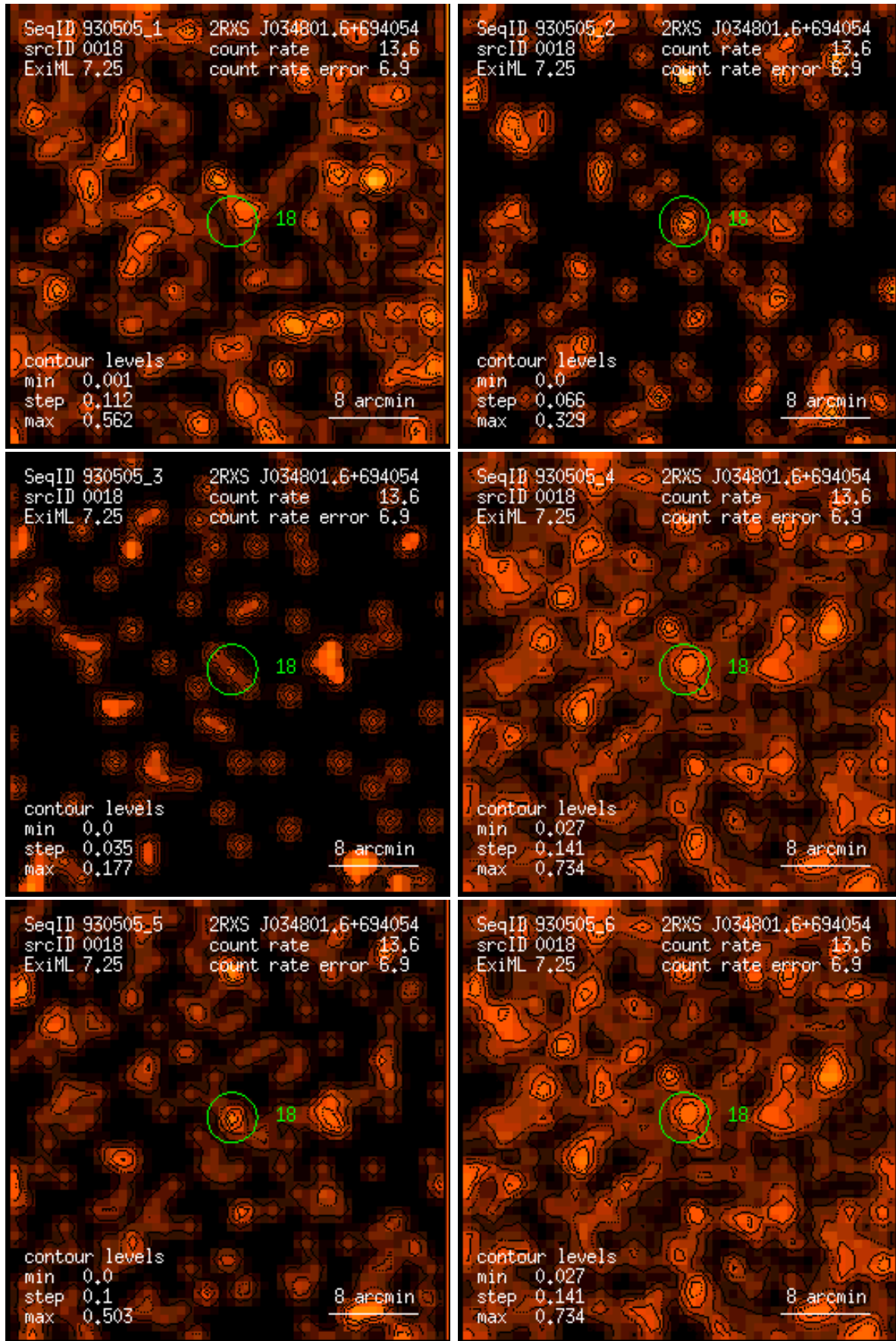
Figure 18: RASS 930505: detection 0018: band rate images, Gaussian filter: (1) PSPC channels 11 – 41, (2) 52 – 90, (3) 91 – 201, (4) 11 – 235, (5) 52 – 201, (6) 11 – 201. Broad band rates in counts/ks. Band rate contour levels in counts/ks/arcmin 2 .
