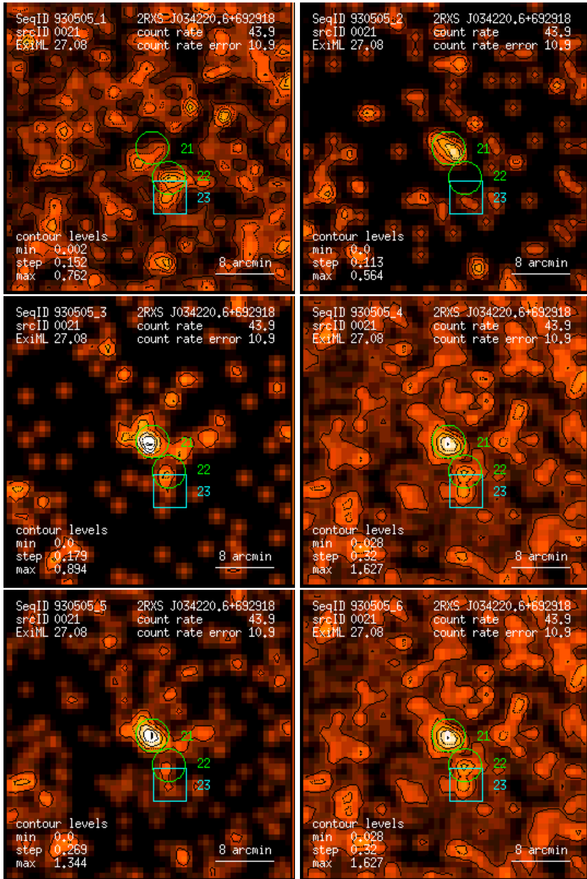
Figure 21: RASS 930505: detection 0021: band rate images, Gaussian filter: (1) PSPC channels 11 – 41, (2) 52 – 90, (3) 91 – 201, (4) 11 – 235, (5) 52 – 201, (6) 11 – 201. Broad band rates in counts/ks. Band rate contour levels in counts/ks/arcmin 2 .
