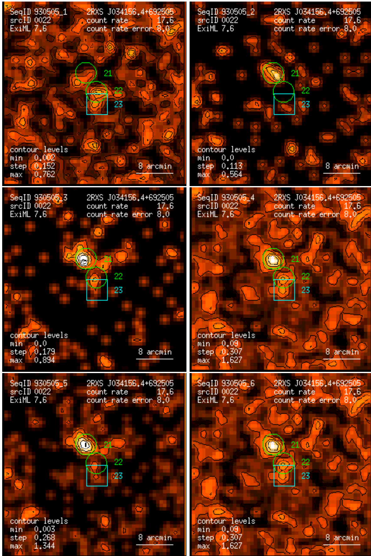
Figure 22: RASS 930505: detection 0022: band rate images, Gaussian filter: (1) PSPC channels 11 – 41, (2) 52 – 90, (3) 91 – 201, (4) 11 – 235, (5) 52 – 201, (6) 11 – 201. Broad band rates in counts/ks. Band rate contour levels in counts/ks/arcmin 2 .
