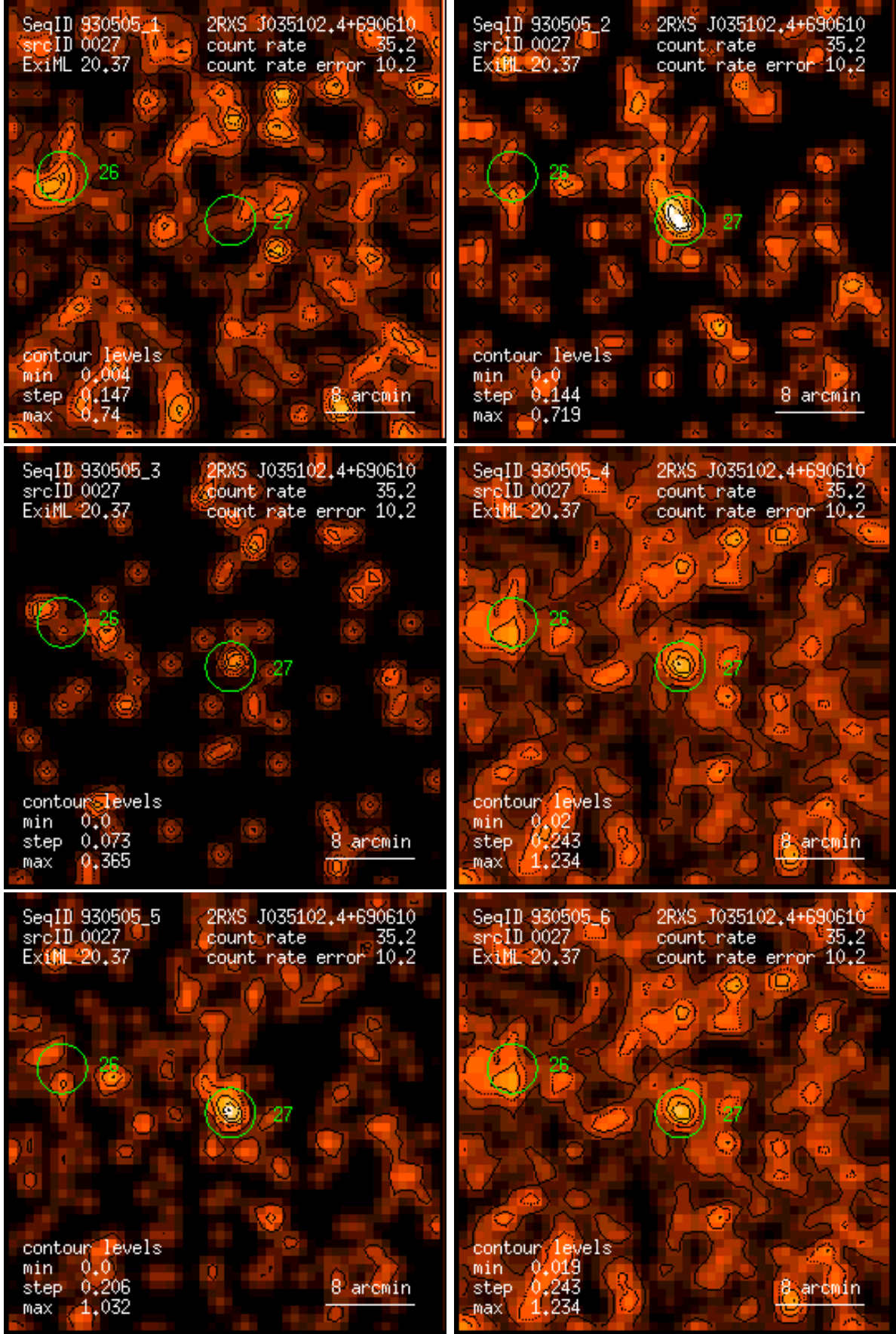
Figure 27: RASS 930505: detection 0027: band rate images, Gaussian filter: (1) PSPC channels 11 – 41, (2) 52 – 90, (3) 91 – 201, (4) 11 – 235, (5) 52 – 201, (6) 11 – 201. Broad band rates in counts/ks. Band rate contour levels in counts/ks/arcmin 2 .
