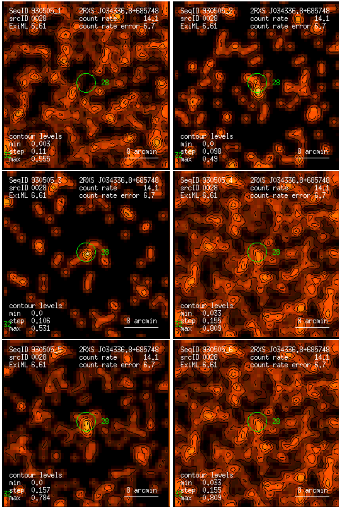
Figure 28: RASS 930505: detection 0028: band rate images, Gaussian filter: (1) PSPC channels 11 – 41, (2) 52 – 90, (3) 91 – 201, (4) 11 – 235, (5) 52 – 201, (6) 11 – 201. Broad band rates in counts/ks. Band rate contour levels in counts/ks/arcmin 2 .
