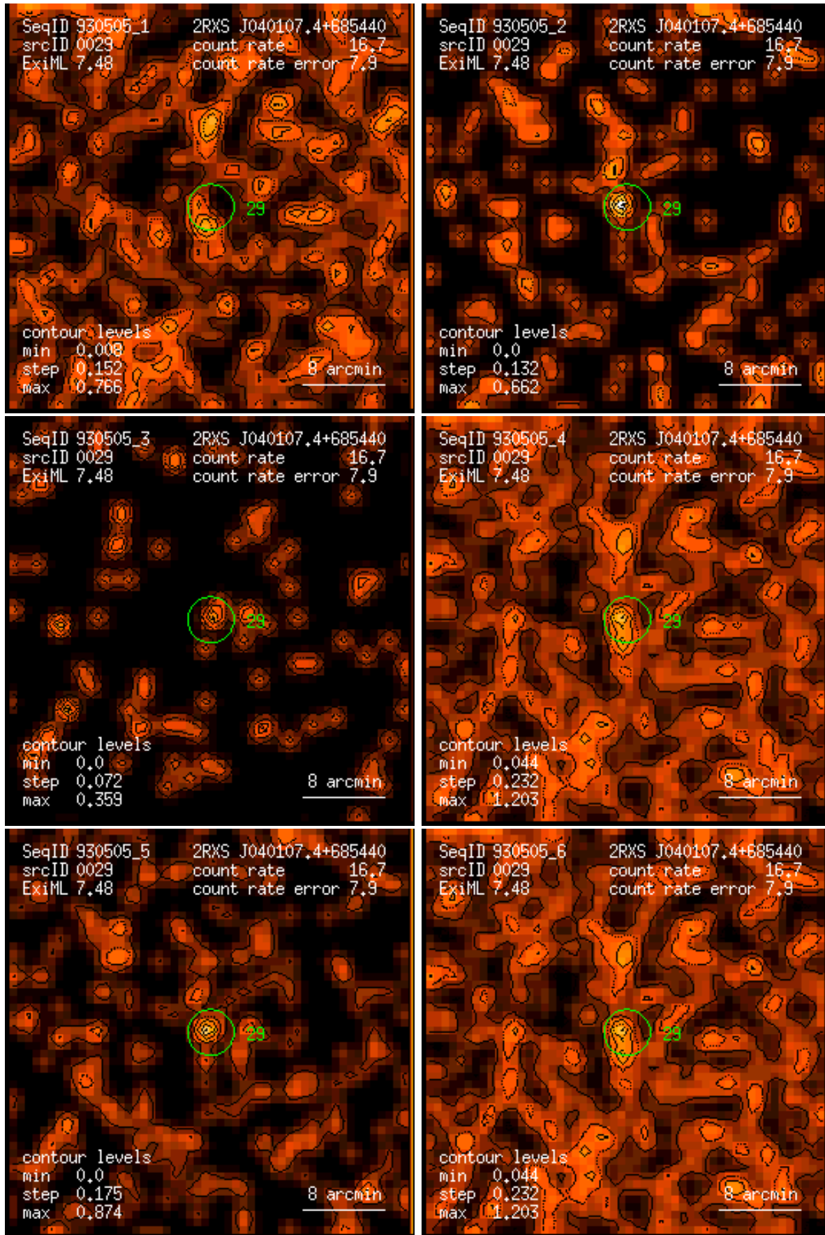
Figure 29: RASS 930505: detection 0029: band rate images, Gaussian filter: (1) PSPC channels 11 – 41, (2) 52 – 90, (3) 91 – 201, (4) 11 – 235, (5) 52 – 201, (6) 11 – 201. Broad band rates in counts/ks. Band rate contour levels in counts/ks/arcmin 2 .
