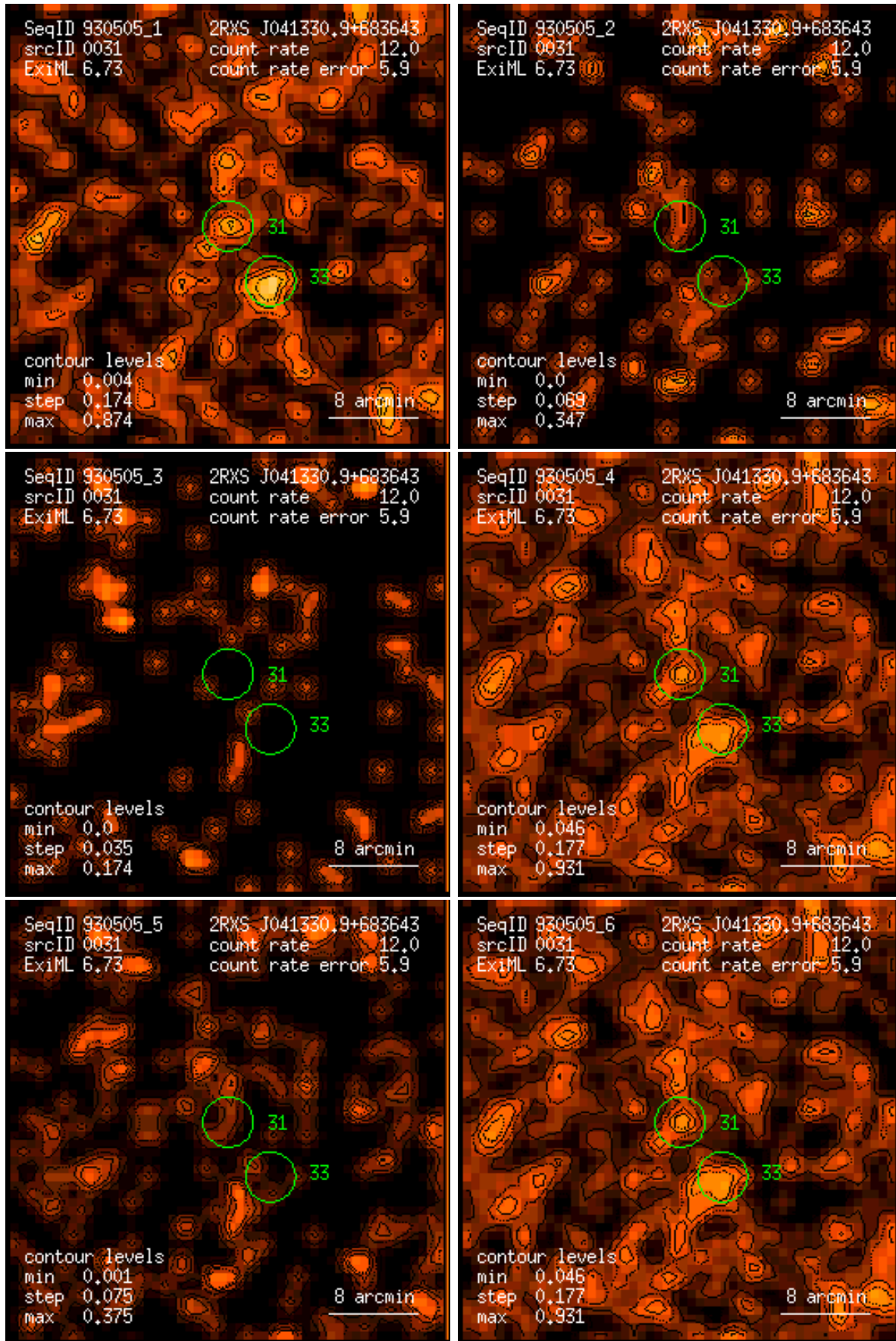
Figure 31: RASS 930505: detection 0031: band rate images, Gaussian filter: (1) PSPC channels 11 – 41, (2) 52 – 90, (3) 91 – 201, (4) 11 – 235, (5) 52 – 201, (6) 11 – 201. Broad band rates in counts/ks. Band rate contour levels in counts/ks/arcmin 2 .
