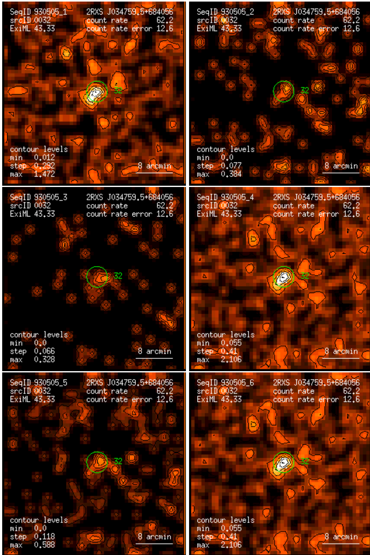
Figure 32: RASS 930505: detection 0032: band rate images, Gaussian filter: (1) PSPC channels 11 – 41, (2) 52 – 90, (3) 91 – 201, (4) 11 – 235, (5) 52 – 201, (6) 11 – 201. Broad band rates in counts/ks. Band rate contour levels in counts/ks/arcmin 2 .
