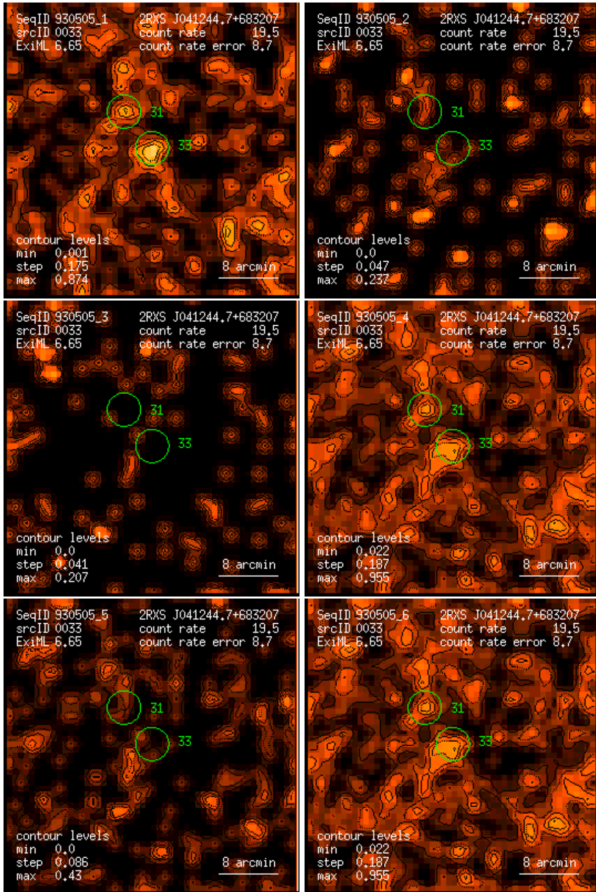
Figure 33: RASS 930505: detection 0033: band rate images, Gaussian filter: (1) PSPC channels 11 – 41, (2) 52 – 90, (3) 91 – 201, (4) 11 – 235, (5) 52 – 201, (6) 11 – 201. Broad band rates in counts/ks. Band rate contour levels in counts/ks/arcmin 2 .
