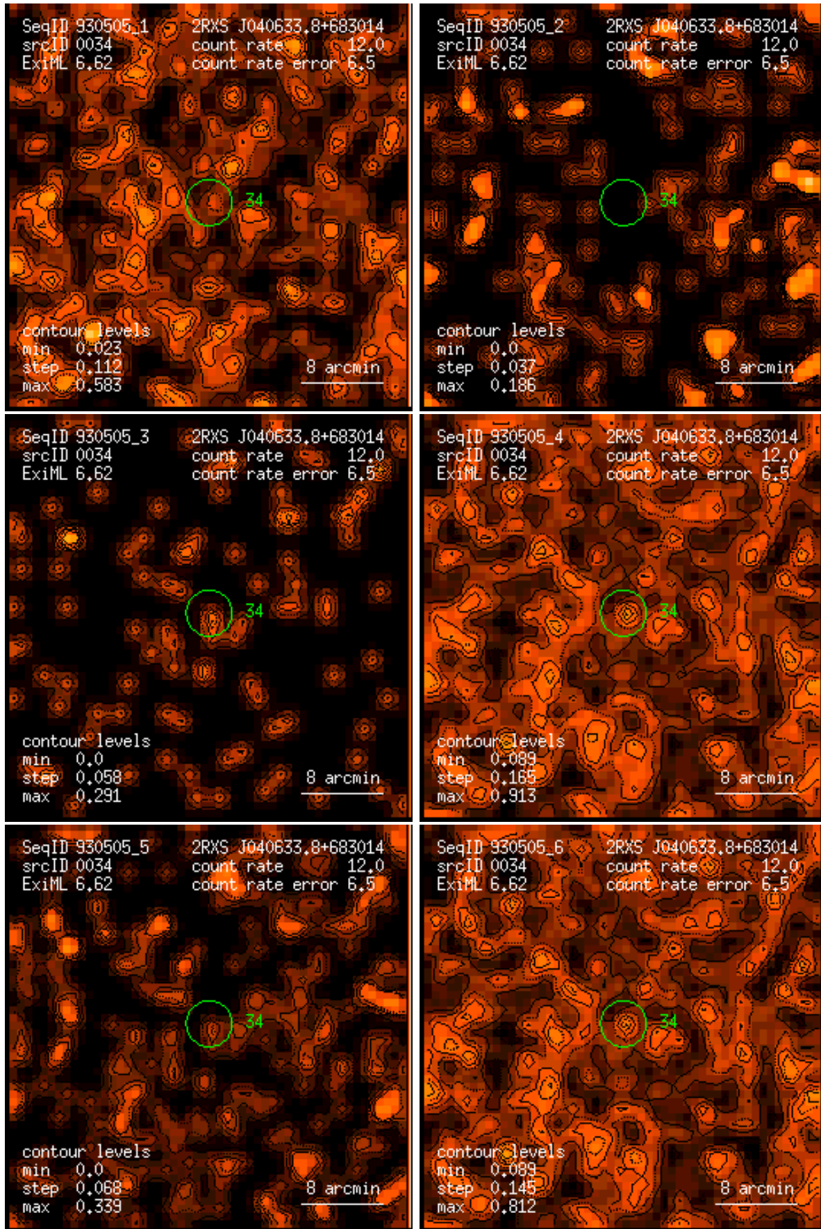
Figure 34: RASS 930505: detection 0034: band rate images, Gaussian filter: (1) PSPC channels 11 – 41, (2) 52 – 90, (3) 91 – 201, (4) 11 – 235, (5) 52 – 201, (6) 11 – 201. Broad band rates in counts/ks. Band rate contour levels in counts/ks/arcmin 2 .
