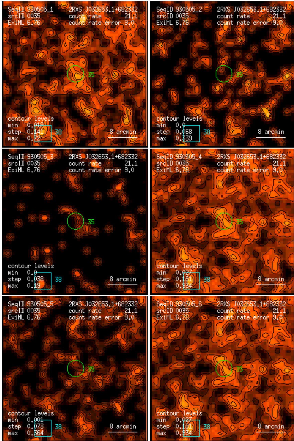
Figure 35: RASS 930505: detection 0035: band rate images, Gaussian filter: (1) PSPC channels 11 – 41, (2) 52 – 90, (3) 91 – 201, (4) 11 – 235, (5) 52 – 201, (6) 11 – 201. Broad band rates in counts/ks. Band rate contour levels in counts/ks/arcmin 2 .
