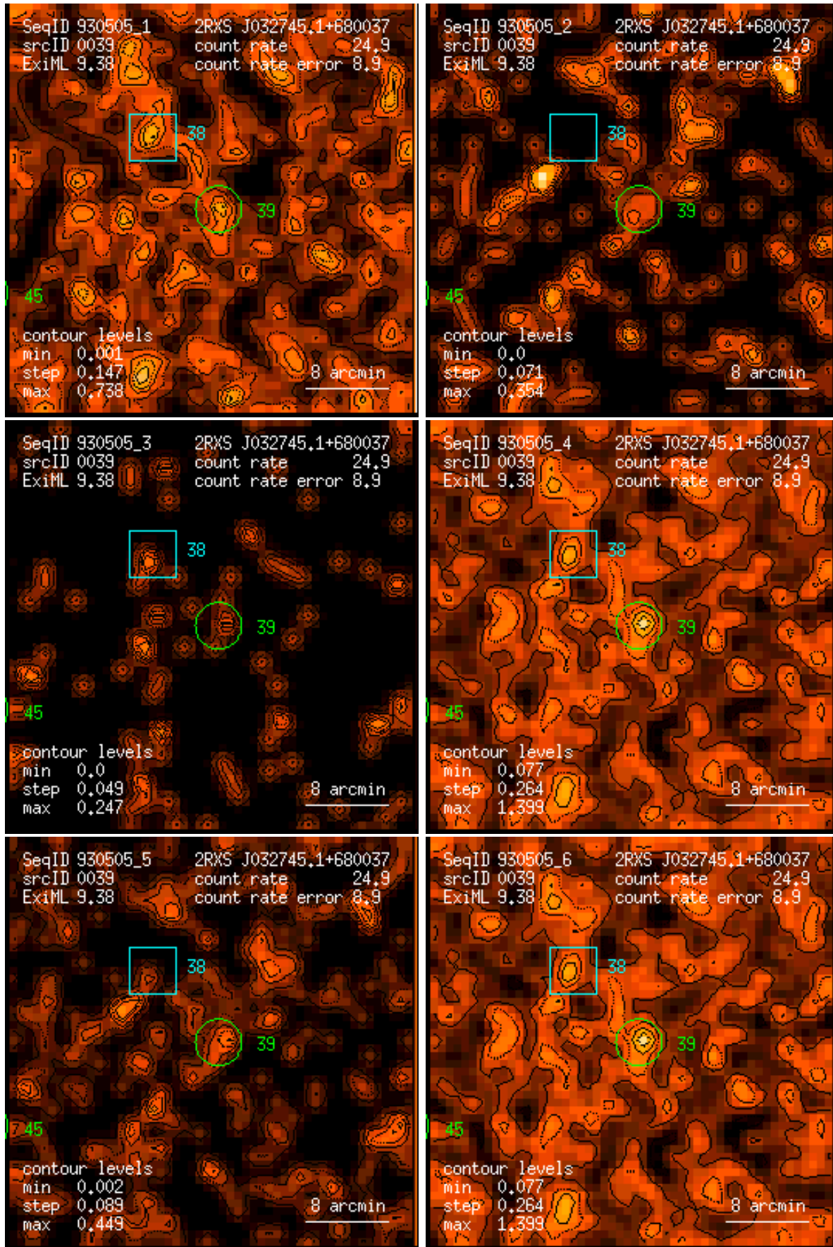
Figure 39: RASS 930505: detection 0039: band rate images, Gaussian filter: (1) PSPC channels 11 – 41, (2) 52 – 90, (3) 91 – 201, (4) 11 – 235, (5) 52 – 201, (6) 11 – 201. Broad band rates in counts/ks. Band rate contour levels in counts/ks/arcmin 2 .
