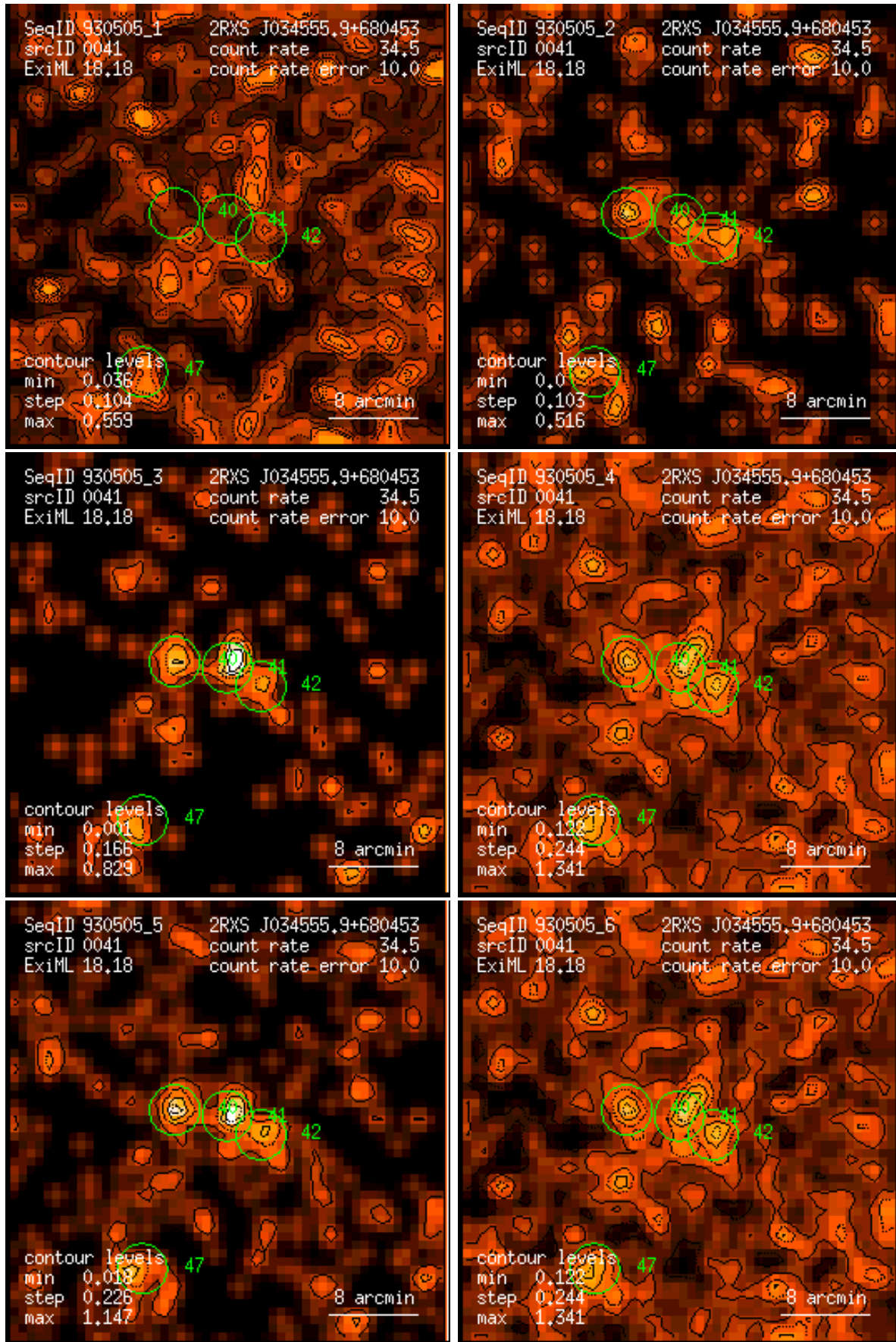
Figure 41: RASS 930505: detection 0041: band rate images, Gaussian filter: (1) PSPC channels 11 – 41, (2) 52 – 90, (3) 91 – 201, (4) 11 – 235, (5) 52 – 201, (6) 11 – 201. Broad band rates in counts/ks. Band rate contour levels in counts/ks/arcmin 2 .
