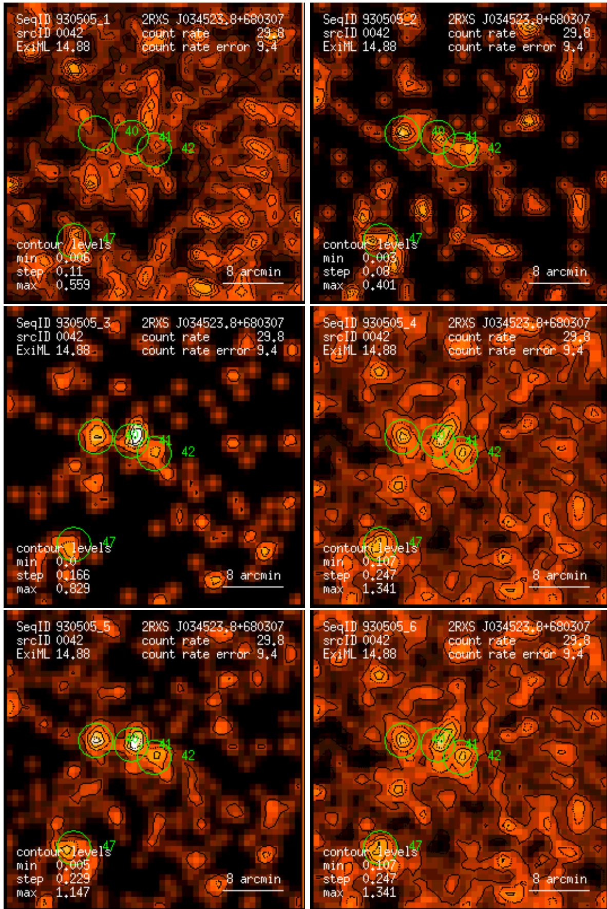
Figure 42: RASS 930505: detection 0042: band rate images, Gaussian filter: (1) PSPC channels 11 – 41, (2) 52 – 90, (3) 91 – 201, (4) 11 – 235, (5) 52 – 201, (6) 11 – 201. Broad band rates in counts/ks. Band rate contour levels in counts/ks/arcmin 2 .
