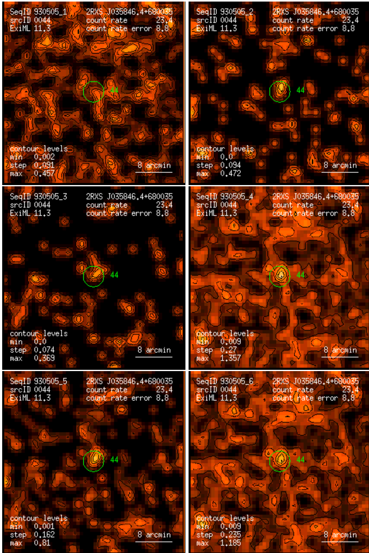
Figure 44: RASS 930505: detection 0044: band rate images, Gaussian filter: (1) PSPC channels 11 – 41, (2) 52 – 90, (3) 91 – 201, (4) 11 – 235, (5) 52 – 201, (6) 11 – 201. Broad band rates in counts/ks. Band rate contour levels in counts/ks/arcmin 2 .
