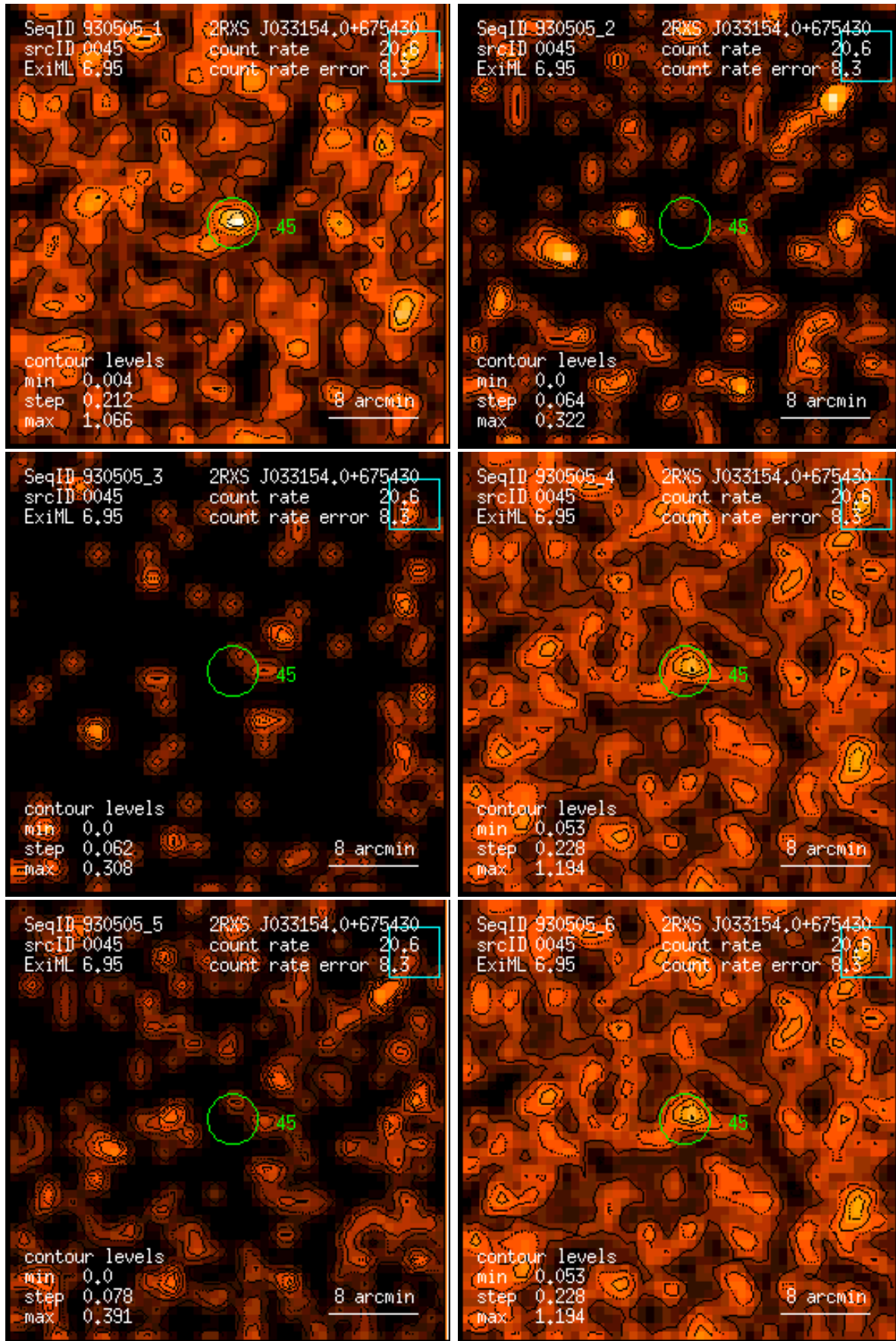
Figure 45: RASS 930505: detection 0045: band rate images, Gaussian filter: (1) PSPC channels 11 – 41, (2) 52 – 90, (3) 91 – 201, (4) 11 – 235, (5) 52 – 201, (6) 11 – 201. Broad band rates in counts/ks. Band rate contour levels in counts/ks/arcmin 2 .
