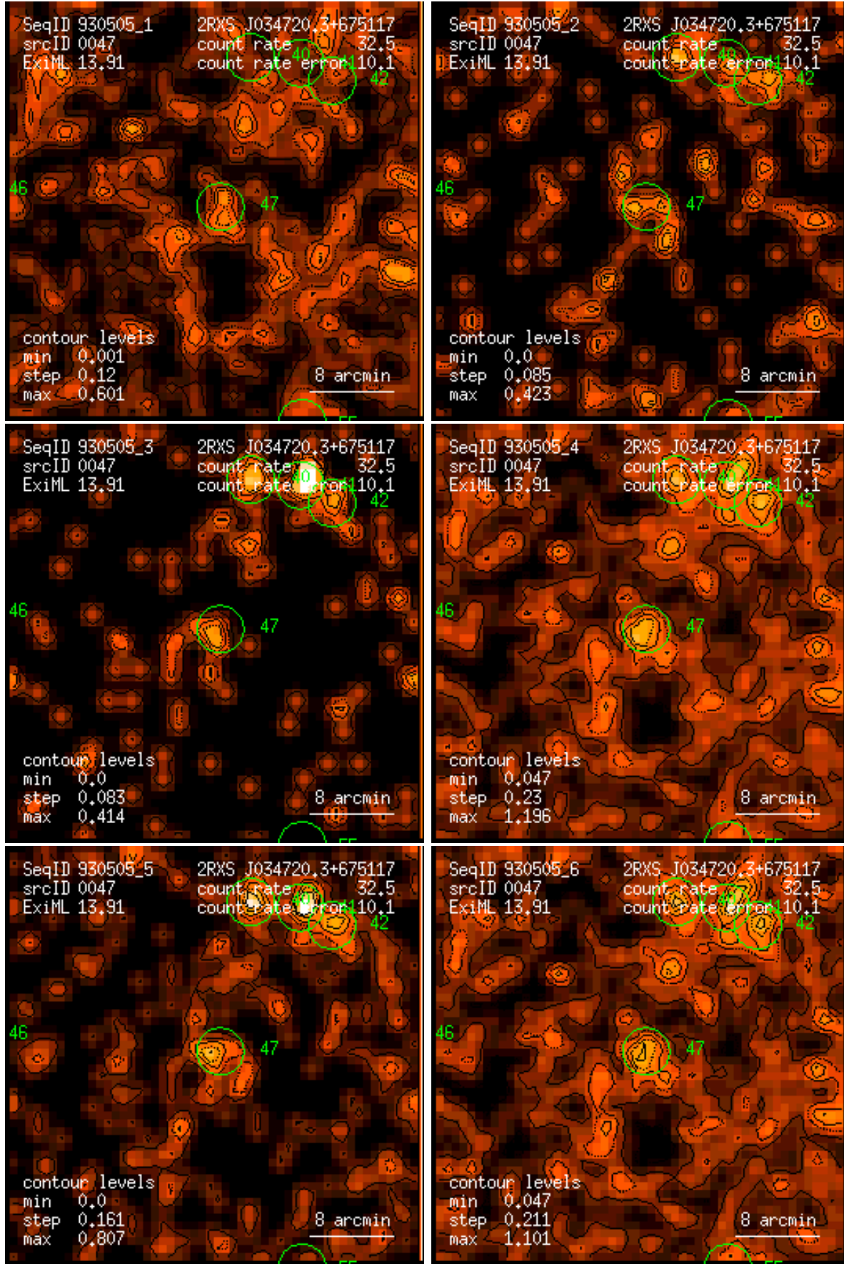
Figure 47: RASS 930505: detection 0047: band rate images, Gaussian filter: (1) PSPC channels 11 – 41, (2) 52 – 90, (3) 91 – 201, (4) 11 – 235, (5) 52 – 201, (6) 11 – 201. Broad band rates in counts/ks. Band rate contour levels in counts/ks/arcmin 2 .
